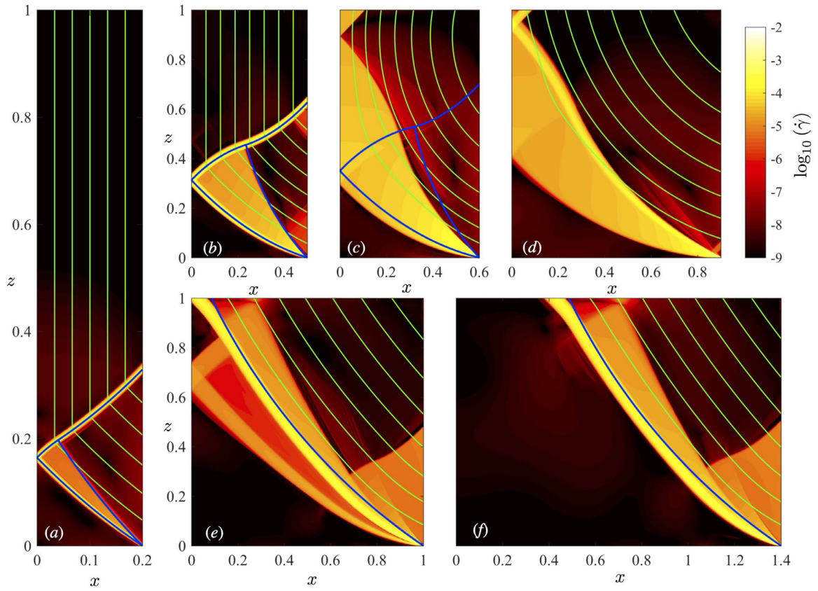
Fig. 12. Strain-rate invariant plotted logarithmically as a density on the (x, z) -plane for solutions with B = 0.99B_c and t = Re = 0 (A.2), at the values of X_0 indicated by the x -axis. Also shown are a selection of streamlines. In (a)–(c), the darker (blue) lines indicate the border of the plastic region and expansion fan of the corresponding slipline solutions (Appendix D). In (e) and (f), the darker (blue) lines indicate the circular failure surface of the lower bound solution. (For interpretation of the references to colour in this figure legend, the reader is referred to the web version of this article.)
