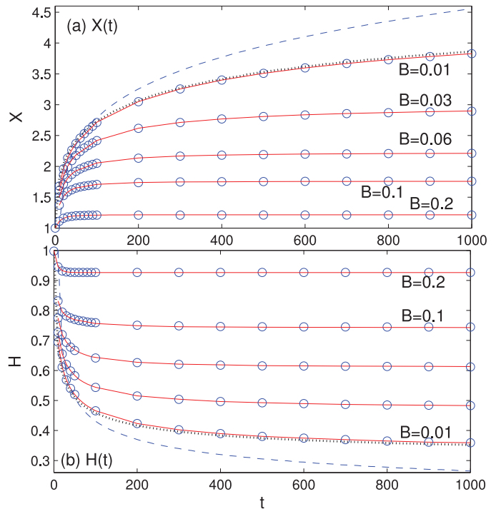
Fig. 4. (a) Front position X(t) and (b) central depth H(t) = h(0, t) for Bingham dambreaks with a square initial block ( X_0 = 1 ) and the values of B indicated. The dashed lines show the Newtonian results. For the viscoplastic cases, the circles show the result using the augmented-Lagrangian scheme and the lines indicate the result with a regularized constitutive law. The dotted lines show the prediction of the leading-order shallow-layer asymptotics for B = 0.01 .
