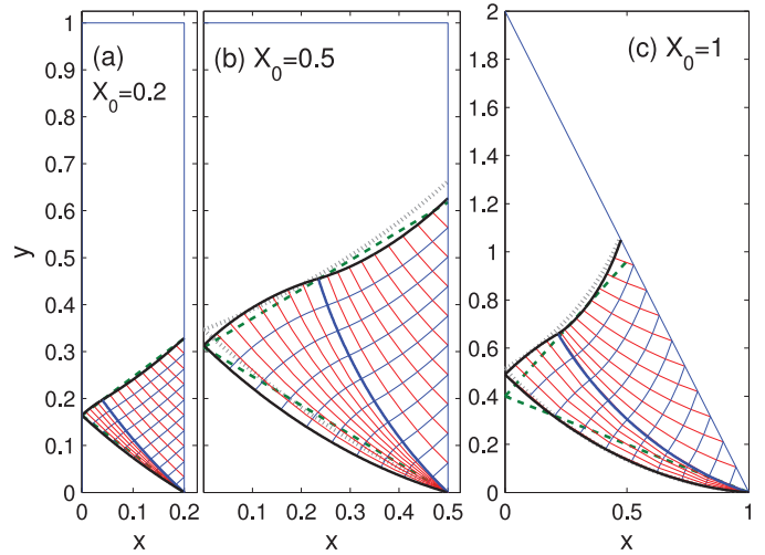
Fig. D.19. Slipline solutions for a rectangle with (a) X_0 = 0.2 and (b) X_0 = 0.5 , and a triangle with X_0 = 1 . The dashed and dotted lines indicate the lower bound and its improvement of D.2.
