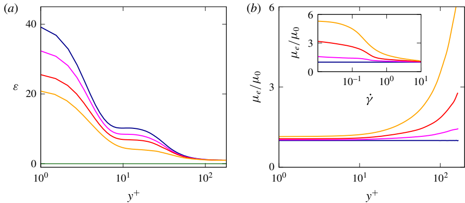
FIGURE 12. (Colour online) Wall-normal profiles of (a) the turbulent dissipation \varepsilon = \mu \partial u'_i / \partial x_j \partial u'_i / \partial x_j in wall units and of (b) the shear effective viscosity \mu_e . The colour scheme is the same as in figure 6. The inset figure in (b) shows \mu_e as a function of the shear rate \dot{\gamma} .
