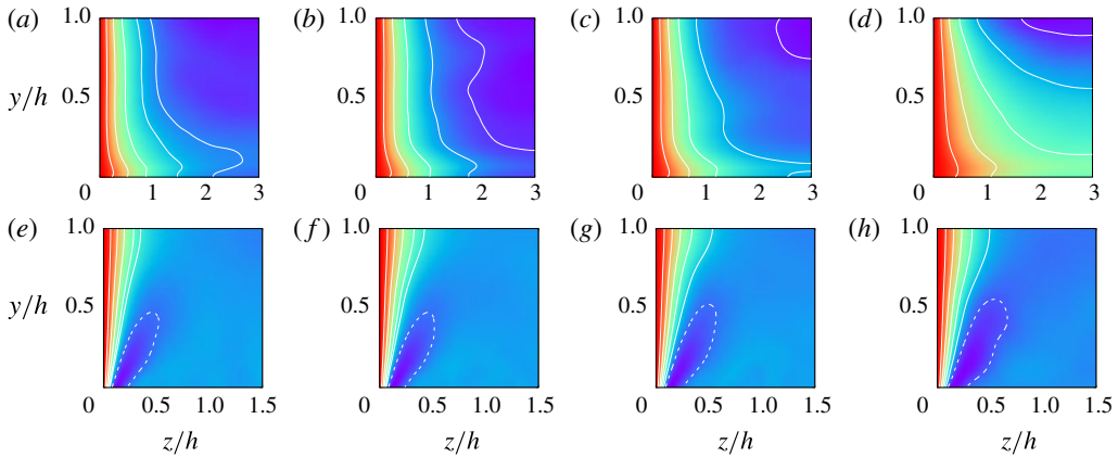
FIGURE 17. (Colour online) Stack of two-point velocity autocorrelation functions across the channel \mathcal{R}_{ii}(y) . (a–d) Shows the streamwise autocorrelation function of the streamwise velocity \mathcal{R}_{11} , while (e–h) the spanwise autocorrelation function of the wall-normal velocity \mathcal{R}_{22} . The Bingham numbers increase from left to right ( Bi = 0, 0.28, 0.7 and 1.4 ). The solid and dashed lines correspond to positive and negative values of autocorrelation, ranging from -0.1 to 0.9 with a step of 0.2 between two neighbouring lines. The colour scale ranges from -0.1 (purple) to 1.0 (red).
