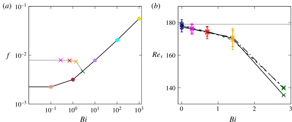
FIGURE 5. (Colour online) (a) Fanning friction factor f as a function of the Bingham number Bi for Re_b = 2800 and \beta = 0.95 . The points on the black line correspond to laminar flows, while those on the grey line to turbulent flows. (b) The friction Reynolds number Re_\tau as a function of the Bingham number Bi , with the vertical error bars measuring the variance of Re_\tau . The dashed, dash-dotted and solid lines are used for \beta = 0.25, 0.5 and 0.95 , respectively. The Reynolds number is equal to Re_b = 2800 for all cases. The blue, magenta, red, orange and green colours are used for the turbulent cases with Bi = 0, 0.28, 0.7, 1.4 and 2.8 , respectively, while the colour scheme for the laminar results is the same as in figure 3.
