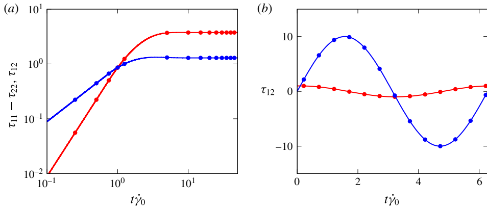
FIGURE 2. (Colour online) (a) Time evolution of \tau_{11} - \tau_{22} (red) and \tau_{12} (blue) in a stationary shear flow. The stress components are normalized with \mu_0 \dot{\gamma} . (b) Time evolution of the shear stress \tau_{12} in an oscillating shear flow with Bi = 0 (red) and Bi = 300 (blue). The stress components are normalized with \mu_0 \gamma_0 \omega_0 . In both panels, solid lines are used for our numerical results and symbols for the analytical solution reported by Saramito (2007).
