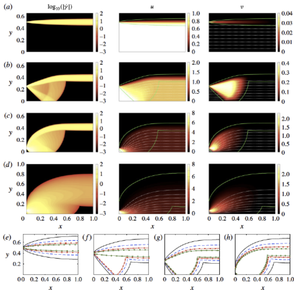
FIGURE 4. (Colour online) Intrusions for (a) y_I = 2^{-1} , (b) y_I = 2^{-2} and (c) y_I = 2^{-4} , all with Bi = 2048 and showing only the upper half of the domain owing to symmetry at y = 0 . Each row shows density plots of \log_{10}(\dot{\gamma}) (left), u(x, y) (centre) and v(x, y) (right); the dotted (white) lines show a selection of streamlines and the solid (green) line shows the yield surfaces. (d) The same set of plots for y_I = 2^{-4} and Bi = 8 ; the flow is similar to the larger- Bi solutions, but without distinct shear layers. (e–h) Yield surfaces for the same inlet widths as (a–c), together with the borderline case at y_I = 0.4 , for Bi = 32 (solid), Bi = 128 (dashed), Bi = 512 ( \square ) and Bi = 2048 ( \circ ).
