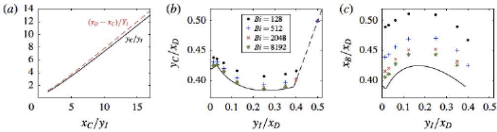
FIGURE 9. (Colour online) Plot of (a) y_C/y_I and (x_D - x_C)/y_I against x_C/y_I , then (b) y_C/x_D and (c) x_B/x_D , both against y_I/x_D . The lines show the slipline solutions and the symbols, which correspond to different values of Bi as indicated, show the numerical solutions. See figure 7 for the locations of A, B, C and D.
