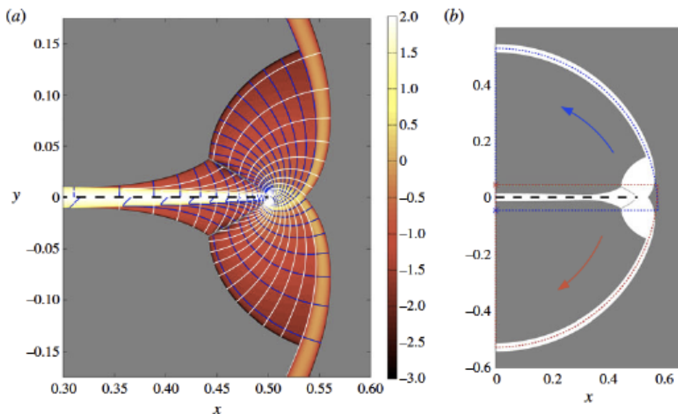
FIGURE 12. (Colour online) Features of the flow near the front of the plate (black dashed) for Bi = 2048 . (a) Sliplines (contours of p \pm 2Bi\theta ), as calculated from the numerical solutions, overlaid on a density map of \log_{10} \dot{\gamma} . Grey regions indicate rigid plugs. (b) The centre of rotation (stars) and one quarter of the arc of rotation (dashed), for the counter-rotating plugs above and below the plate.
