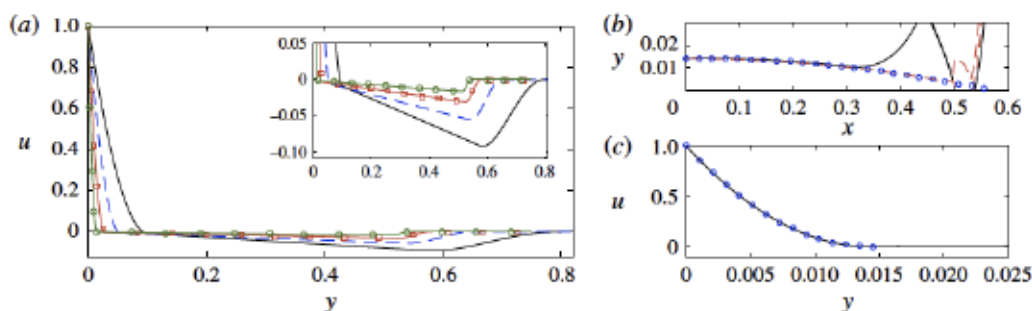
FIGURE 13. (Colour online) (a) Horizontal velocity profiles at x=0 for Bi=32 (black), Bi=128 (blue dashed), Bi=512 (red squares) and Bi=2048 (green circles). The inset shows the velocity across the rigid plug and outer circular boundary layer in more detail. (b,c) Details of the numerical solution for Bi=2048 : (b) the yield surface (black solid) and a contour of \dot{\gamma}=1 (red dashed), which approximately demarcates the edge the viscoplastic boundary layer; and (c) the horizontal velocity profile at x=0 . Circles show the asymptotic predictions from (5.9), (5.4) and (5.10), using the measured values of \Omega , R and y_e .
