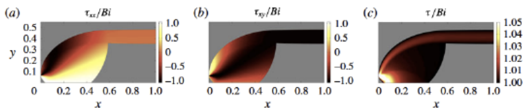
FIGURE 6. (Colour online) Further details of the stress field for the intrusion with y_l = 2^{-4} and Bi = 2048 , which was shown in figure 4(c): density plots of (a) \tau_{xx}/Bi , (b) \tau_{xy}/Bi and (c) \tau/Bi . In view of the indeterminacy of the stress field over the rigid parts of the flow, the plugs are shaded grey.
