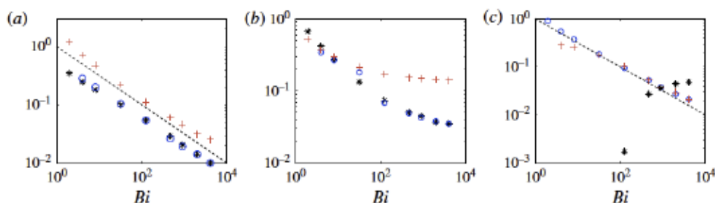
FIGURE 11. (Colour online) Data as a function of Bi . (a) Boundary-layer width at x = 0 for the layer against the plate (*) and for the circular shear layer (red +). (b) Characteristic lengths of the plastic region: horizontal length in front of the tip of the plate x_a - (1/2) (*); maximum height y_b of the stress discontinuity above the plate (blue o); and maximum height y_p of the plastic region (red +). (c) Properties of the rotating plugs as defined in (5.11a,b): y_c (*); R - y_c - (1/2) (blue o); and Bi^{-1/2}\Omega (red +). The dashed lines show Bi^{-1/2} and the (blue) circles in (a) plot the prediction in (5.10).
