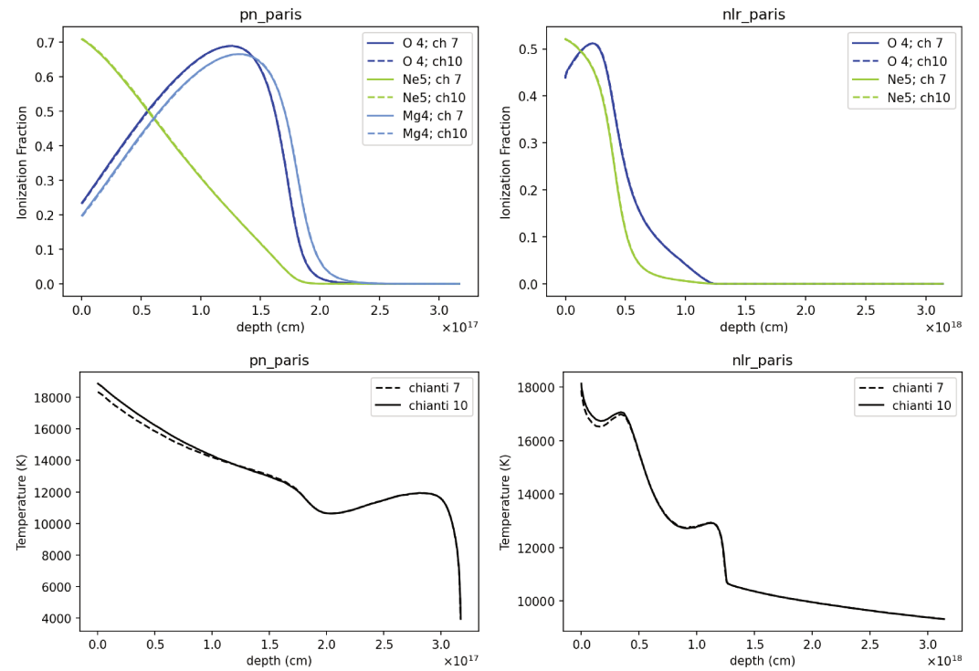
Figure 5. CLOUDY outputs of the pn_paris and nlr_paris test simulations.
