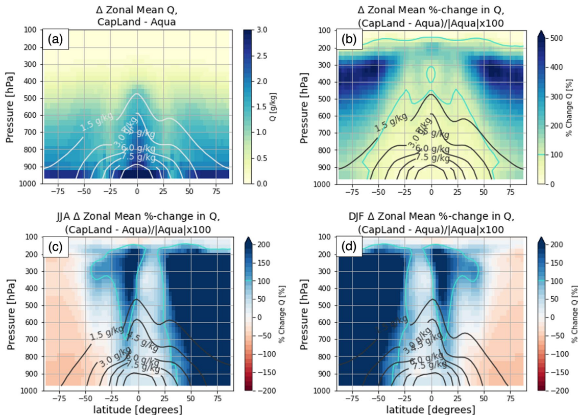
Fig. 9 Difference (CapLand—Aqua) in zonally averaged a annual mean specific humidity [g/kg] is shown in shading, with the climatological specific humidity [g/kg] from Aqua shown in white contours. (b–c) show the percent change specific humidity for b the annual
