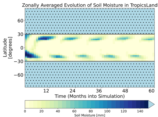
Fig. 16 Hovmöller plot showing the evolution of zonally averaged soil moisture for the first 5 years of the TropicsLand simulation [mm]. Ocean areas are indicated by light blue shading with stippling
