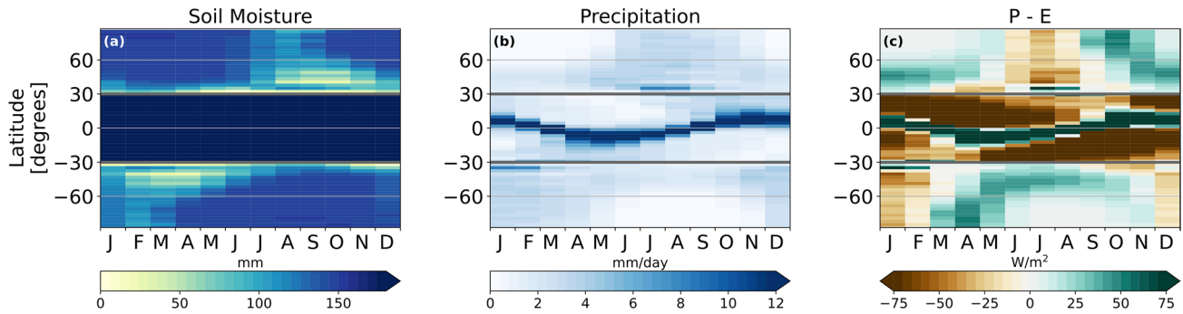
Fig. 18 Zonally averaged a soil moisture [mm], b precipitation [mm/day], and c precipitation-evaporation [ \text{W/m}^2 ] over the course of the year for the CapLand simulation. Dark gray lines at 30^\circ N/S indicate the continental/ocean boundary
