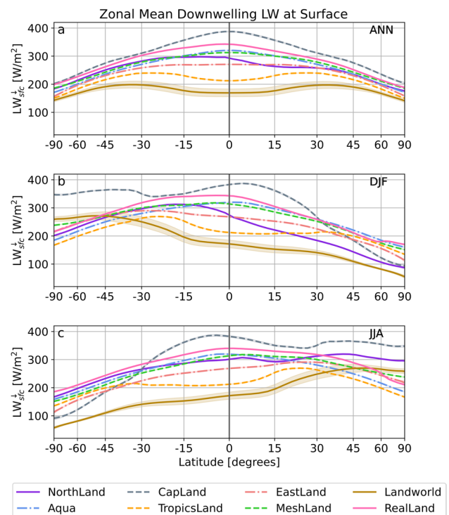
Fig. 17 Zonally averaged downwelling longwave radiation at the surface ( LW_{sfc}^l , in W/m^2 ) for a the annual mean, b December–January–February, and c June–July–August for each continental configuration. Shading indicates \pm 1\sigma of interannual variability
