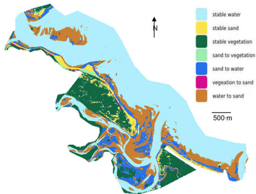
Figure 11. Image analysis (classification's overall accuracy of 97%) using high-resolution satellite photographs shows how depositional environments at the study area changed from 2017 to 2019 (imagery is from PlanetScope satellite).
