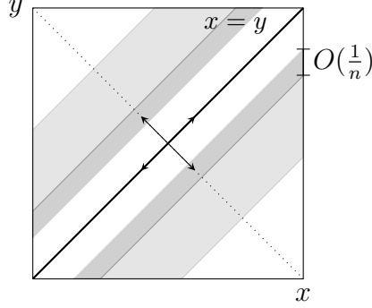
FIGURE 9. Expansion of the set A_n (given in gray) under the map F . The thick, black line represents the line of maximization. Arrows indicate uniform expansion under F in all directions.
