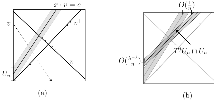
FIGURE 1. (a) The set U_n and line L for L not aligned with v^- or v^+ . (b) Iterations T^jU_n and their intersections with U_n .
