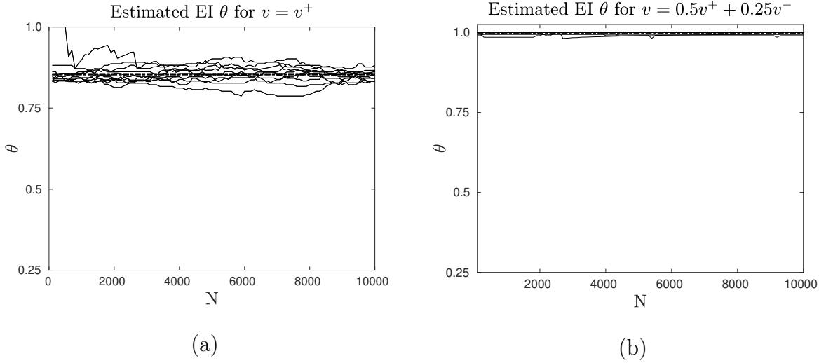
FIGURE 13. Extremal index \theta estimation (10 different realizations, t = 10^4 ) for Arnold's cat map with \varphi(x) = -\log d(x, L) where (a) L = v^+ and (b) L = 0.5v^+ + 0.25v^- . The marked line indicates the theoretical value of \theta given.
