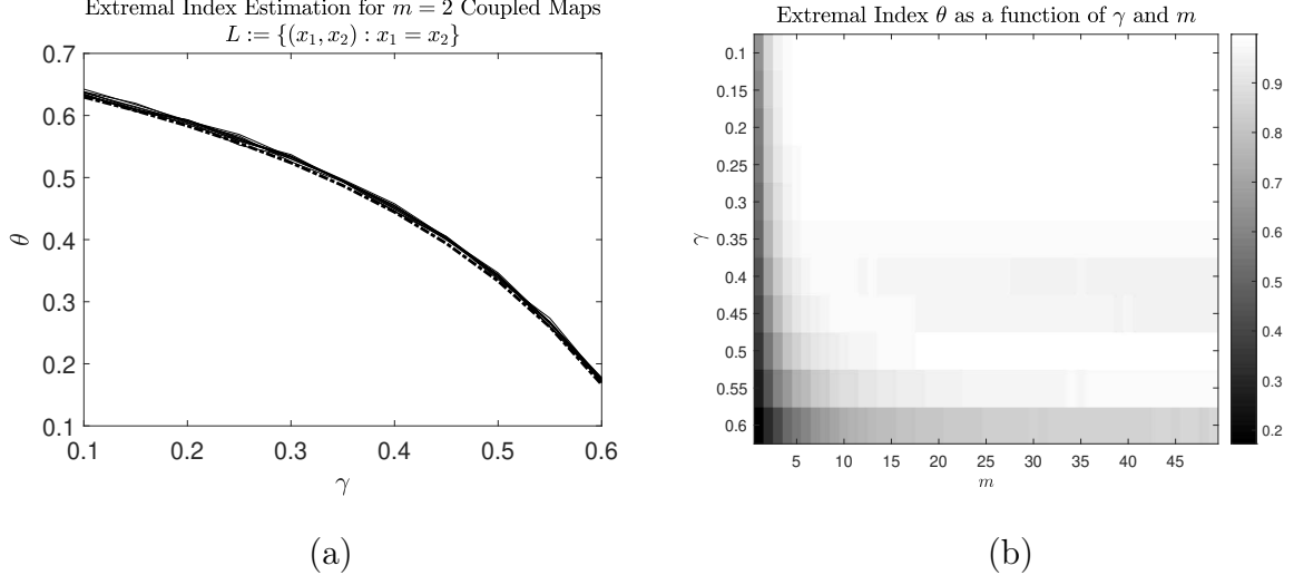
FIGURE 10. Extremal index \theta estimation for the m -coupled map F with \varphi(x) = -\log(\|p^\perp\|) where the set of maximization L = \{(x_1, x_2, \dots, x_m) : x_1 = x_2 = \dots = x_m\} for (a) fixed m and varying \gamma (10 different realizations t = 10^6 ) and (b) varying m and \gamma . (a) The marked line indicates the theoretical value of \theta given. (b) The colorbar indicates the value of 0 \leq \theta \leq 1 for each m and \gamma pair.
