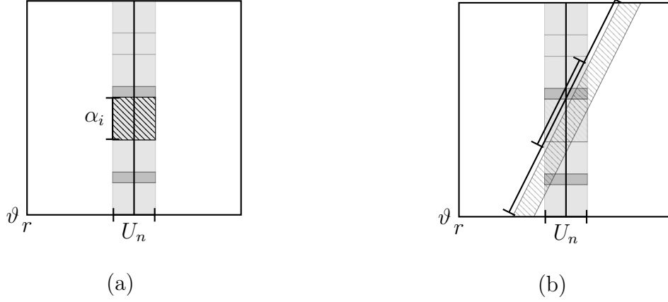
FIGURE 8. (a) Intersection of points with r = r_0 that will not hit a extremal in C \log n iterates. (b) Expansion of a single rectangle of side-length \alpha_i . Lines indicate portion that intersects U_n .
