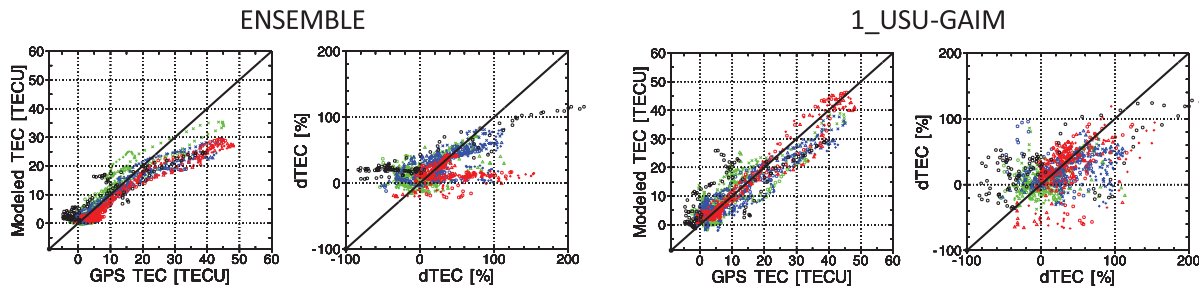
Figure 8. Same as Figure 1 but for only Total Electron Content (TEC) and dTEC[%] from the ensemble of the simulations (ENSEMBLE) and 1_USU-GAIM.
