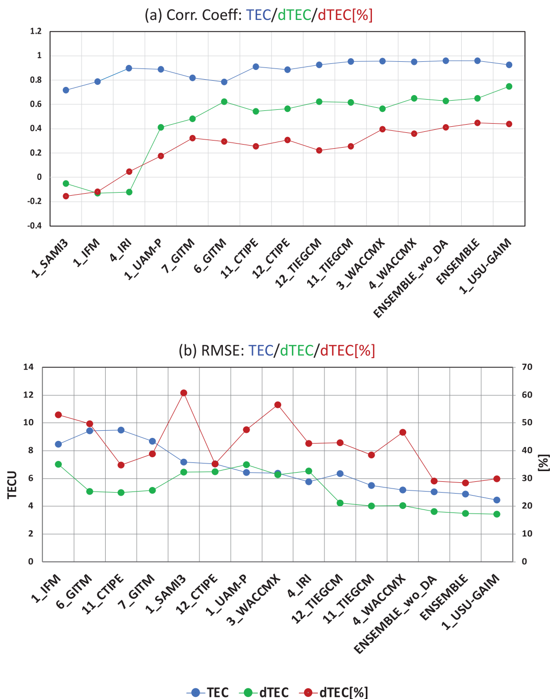
Figure 9. Averaged Correlation coefficient (CC) (a) and root-mean square error (RMSE) (b) over all 12 locations of 13 simulations, the ensemble of them (ENSEMBLE), and the ensemble of 12 simulations excluding 1_USU-GAIM (ENSEMBLE_wo_DA). Blue denotes shifted Total Electron Content (TEC), green and red the change and percentage changes of TEC. CCs are plotted from the smallest to the largest (closer to 1) according to the average of the three averaged CC values of TEC, dTEC, and dTEC[%]. RMSEs are plotted from the largest to the smallest according to the average RMSE for TEC and dTEC.
