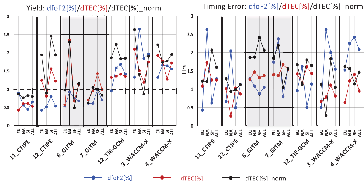
Figure 7. Same as Figure 4 but for Yield (ratio) and absolute of Timing Error ( |TE| = |t_{\text{peak\_model}} - t_{\text{peak\_obs}}| ).
