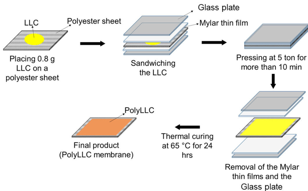
Fig. S1. Schematic representation of polyLLC membrane preparation.
