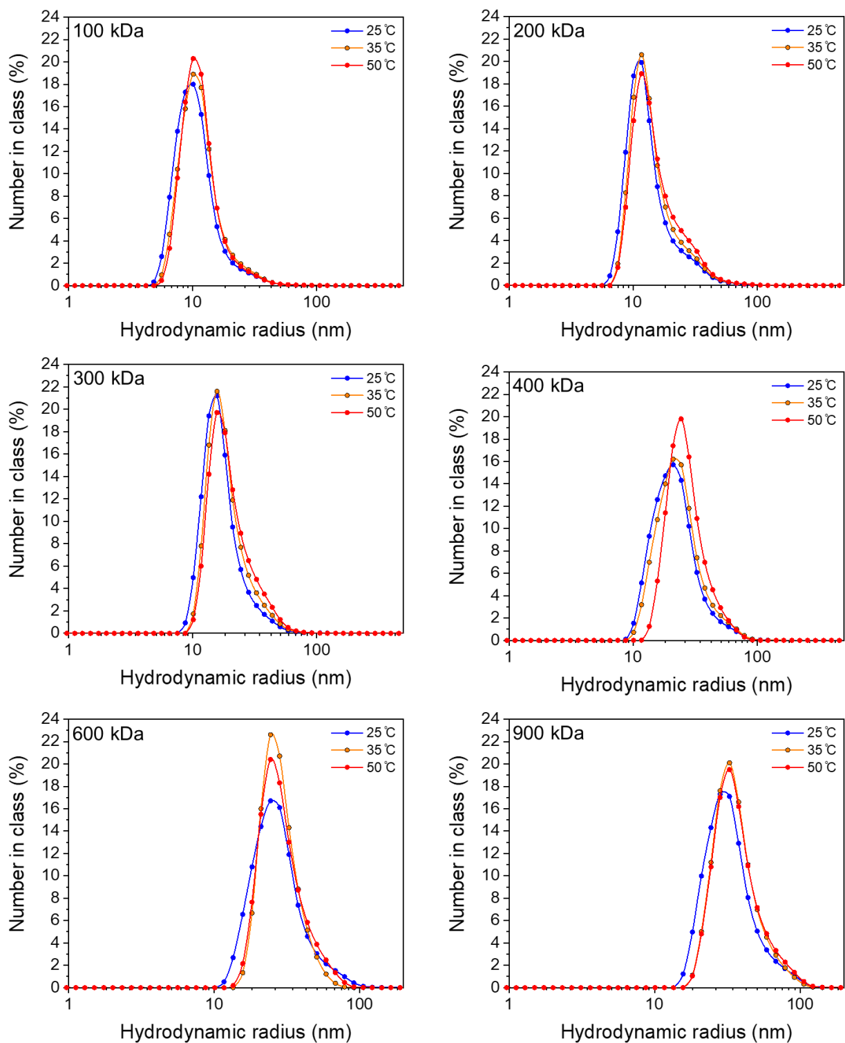
Fig. S2. Temperature-dependent chain size distribution for PEO having different molecular weights.
