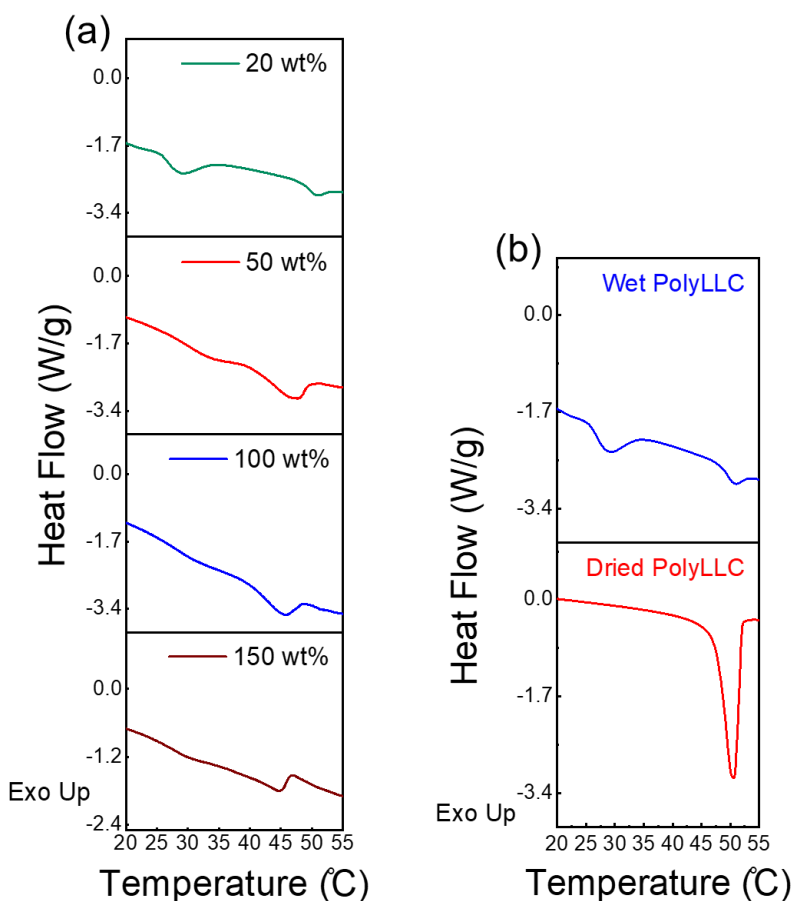
Fig. 9. Results of DSC measurement for (a) polyLLCs containing different cross-linker contents and (b) wet and dried polyLLC containing 20 wt% cross-linker with respect to n BA content.
