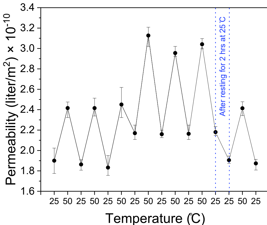
Fig. 5. Reversibility of the water permeability of the polyLLC membrane under several heating-cooling cycles.
