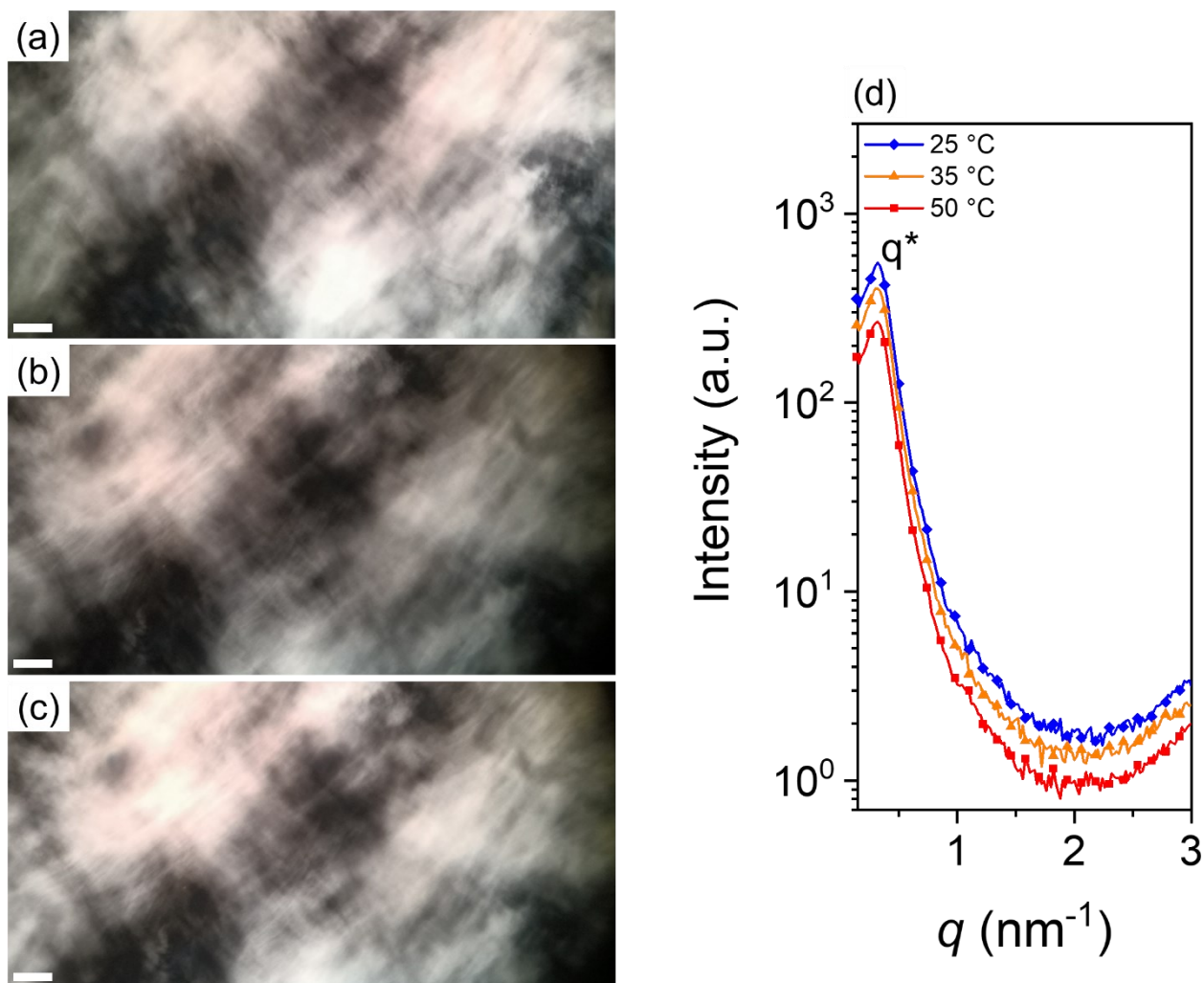
Fig. S3. CPLM images of polyLLC with lamellar structure at (a) 25, (b) 35 and (c) 50 °C (scale bar: 50 \mu\text{m} ). (d) 1D SAXS data for the polyLLC at 25, 35 and 50 °C (the plots are vertically shifted for clarity).
