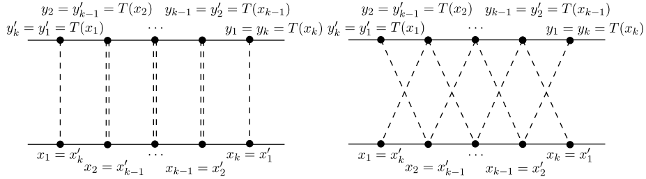
Figure 1. Schematic representation of the sums (4.17) (left) and (4.18) (right). Each dashed line stands for a term c(\cdot, \cdot) .
