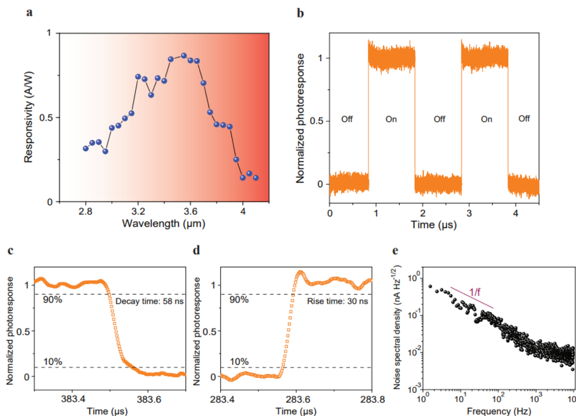
Figure 5. Spectral photoresponse, temporal photoresponse, and noise characterization. (a) Spectral-dependent responsivity of the waveguide-integrated photodetector. (b) Temporal photoresponse of the waveguide-integrated photodetector when the incident light intensity ( \lambda = 3.7 \mu\text{m} , 600 \mu\text{W} ) was modulated at a frequency of 500 kHz. Analysis of the (c) 90–10% fall time and (d) 10–90% rise time. (e) Noise spectral density measured from the waveguide-integrated photodetector.
