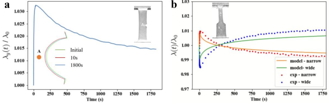
Figure 4: Nonlinear effect of p\text{-}PA_{strong} gel. (a) Time evolution of stretch at A and COD (insert) in SENT specimens (insert) in relaxation tests. (b) Measured strain history versus simulated strain history during relaxation in T -shape specimen (insert) for p\text{-}PA_{strong} gel. \lambda_0 is the local stretch in y direction at measured points at t = 0 .
