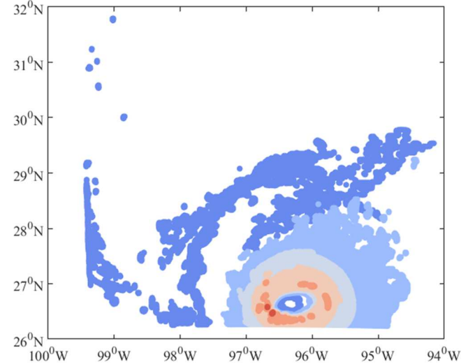
Fig. 3 Wind velocity distribution in the Texas region during Hurricane Harvey.
