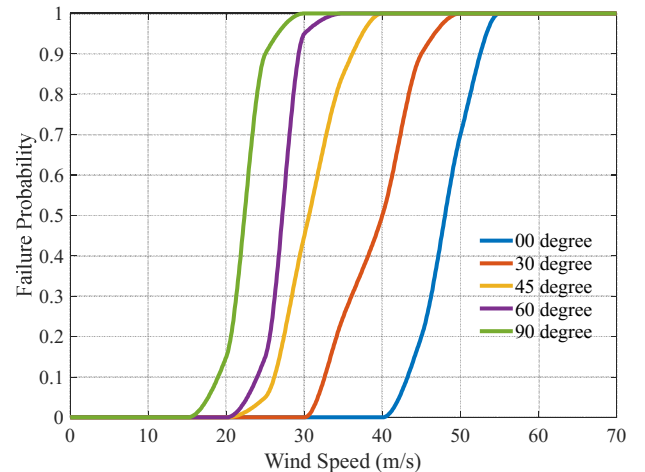
Fig. 4 Transmission tower fragility curves
