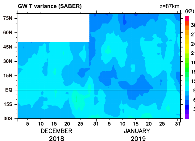
Figure 15. Time-latitude section of gravity wave temperature variances at z = 87\text{ km} from Sounding of the Atmosphere using Broadband Emission Radiometry (SABER) observations for ICSOM-4.
