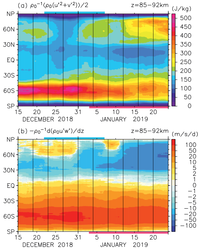
Figure 14. Time-latitude section of gravity wave kinetic energy and zonal momentum flux divergence for z = 85\text{--}92\text{ km} simulated by gravity-wave permitting general circulation model (JAGUAR) for ICSOM-4. The blue bars indicate the warm period in the Arctic stratosphere and the red bars indicate the warm period in the Antarctic upper mesosphere.
