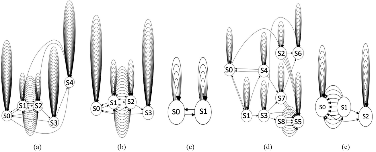
Fig. 4. Mealy machines inferred from the five Bluetooth devices. We have removed the input/output label on each edge for readability. (a) Dell laptop. (b) Raspberry Pi. (c) Keyboard. (d) Android phone. (e) Sony speaker.
