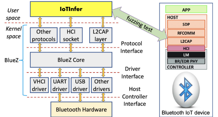
Fig. 3. IoTInfer implementation for Bluetooth L2CAP fuzzing.
