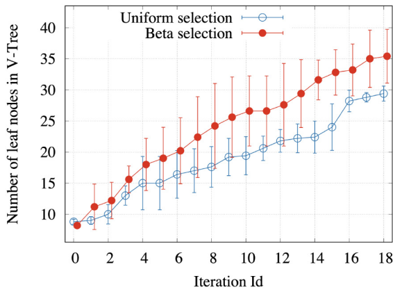
Fig. 6. Performance comparison between uniform selection and Beta selection.
