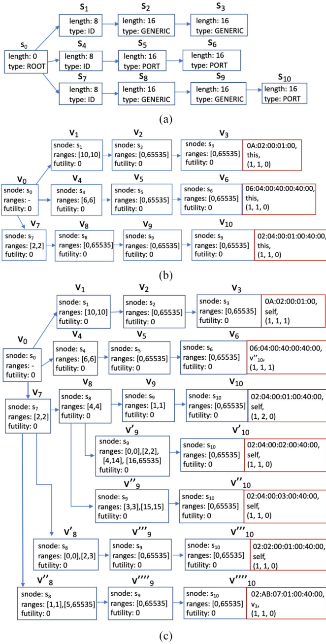
Fig. 1. Illustrating example. The right box of each leaf node includes fields sample , cleader , and ( init_neg , freshness ) in order. (a) STree. (b) VTree after initialization. (c) VTree after one iteration.
