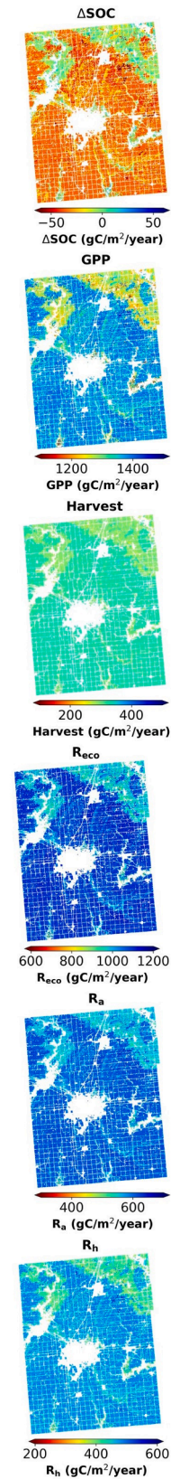
Fig. 8. Simulated carbon budgets and their uncertainties induced by SOC% or Bulk_Density uncertainty in cropland for Champaign County of Illinois.
