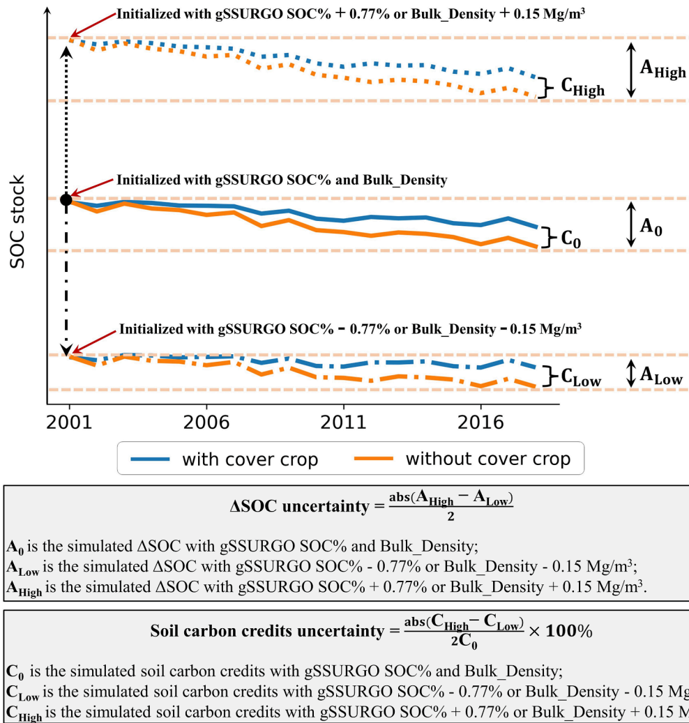
Fig. 1. Illustration of soil carbon change ( \Delta \text{SOC} ), soil carbon credits, and their uncertainty assuming cover crop adopted since the winter of 2000. The solid lines are the changes in model simulated SOC stock initialized with gSSURGO SOC% and Bulk_Density, the dotted lines are the changes in model simulated SOC stock initialized with gSSURGO SOC% + 0.77% or Bulk_Density + 0.15 Mg/m 3 , and the dashdot lines are the changes in model simulated SOC stock initialized with gSSURGO SOC% - 0.77% or Bulk_Density - 0.15 Mg/m 3 . We use \Delta \text{SOC} as an example component of the cropland carbon budgets here, but the uncertainty quantification method also applies to other carbon budget components in Eq. (2).
