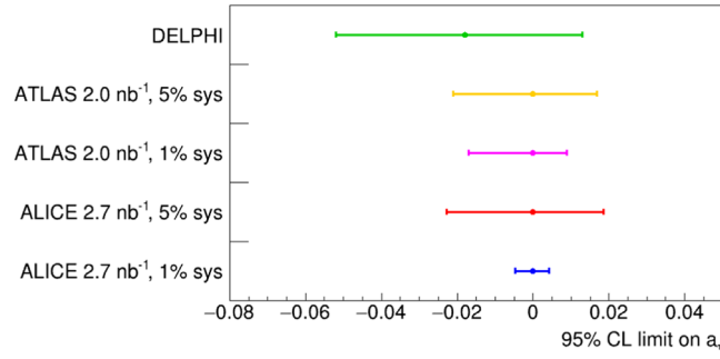
Figure 2. Expected 95% C.L. limits on a_T measurements with available ATLAS/CMS Run 2 data ( 2 \text{ nb}^{-1} ) and with future ALICE data to be collected in 2022 ( 2.7 \text{ nb}^{-1} ) for two different assumptions on systematic uncertainty (1%, 5%) in comparison with DELPHI results [24].
