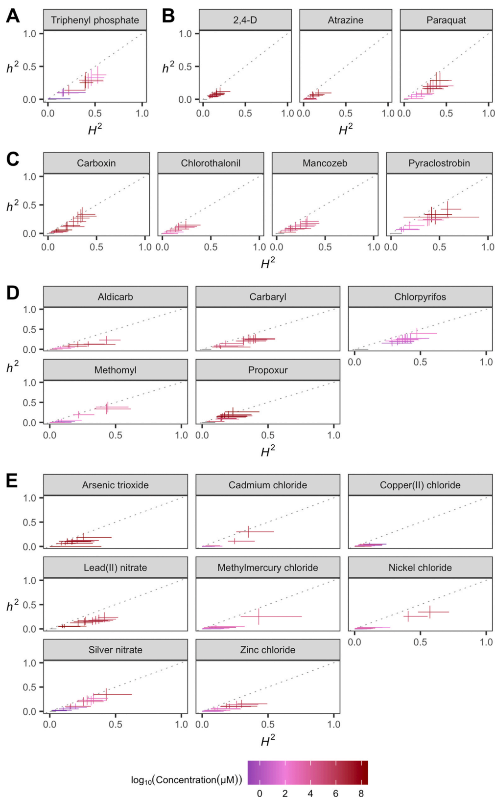
Fig. 5. Variation in toxicant responses is heritable among genetically diverse C. elegans strains. The broad-sense (x-axis) and narrow-sense heritability (y-axis) of normalized animal length measurements was calculated for each concentration of each toxicant (Methods; Broad-sense and narrow-sense heritability calculations). The color of each cross corresponds to the log-transformed exposure for which those calculations were performed. The horizontal line of the cross corresponds to the confidence interval of the broad-sense heritability estimate obtained by bootstrapping, and the vertical line of the cross corresponds to the standard error of the narrow-sense heritability estimate.
