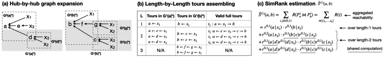
Fig. 4. An example of efficiently estimating \hat{s}^{(1)}(a, b) with graph expansion and length-aware assembling.
