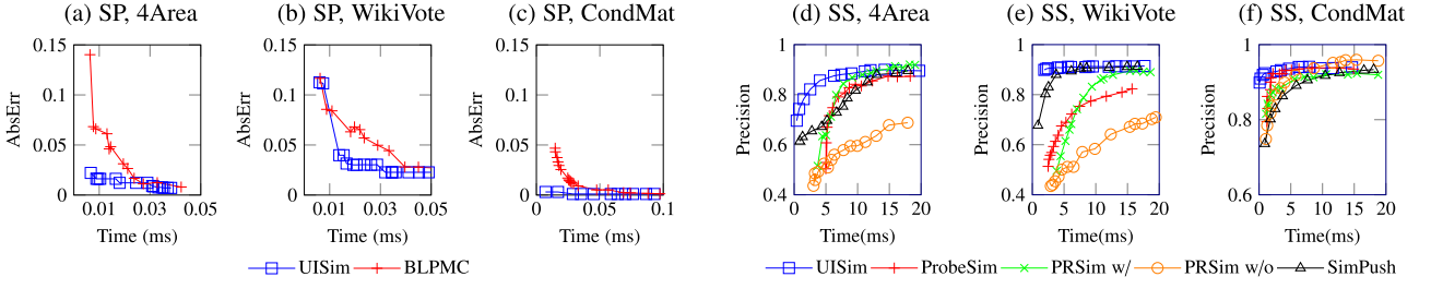
Fig. 8. Comparison of accuracy against time with baselines in single pair (SP) and single source (SS) modes.
