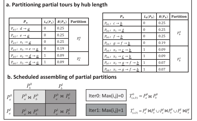
Fig. 3. An example of prioritized generation of full tour partitions with benefit model ( C=0.75 ).
