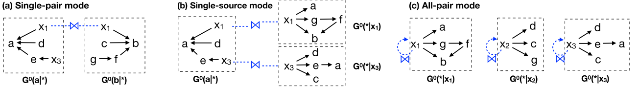
Fig. 5. An example of spanning partial tours in different modes.
