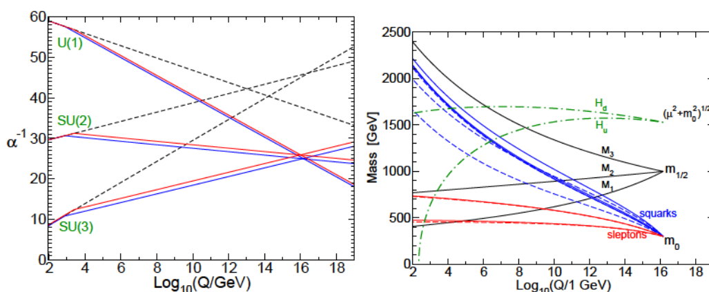
Figure 8.4: RG evolution of scalar and gaugino mass parameters in the MSSM with MSUGRA boundary conditions imposed at Q_0 = 1.5 \times 10^{16} GeV. The parameter \mu^2 + m_{H_u}^2 runs negative, signalling electroweak symmetry breaking.
