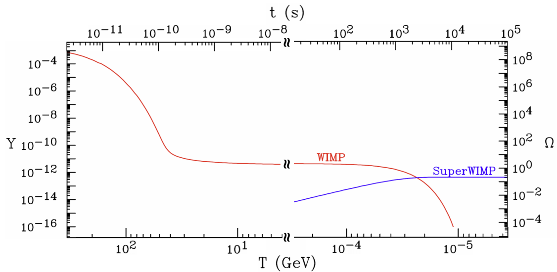
Figure 15: In superWIMP scenarios, WIMPs freeze out as usual, but then decay to superWIMPs, superweakly-interacting massive particles that are the dark matter. This figure shows the WIMP comoving number density Y (left) and the superWIMP relic density (right) as functions of temperature T (bottom) and time t (top). The WIMP is a 1 TeV, S -wave annihilating particle with lifetime 10^3 s, and the superWIMP has mass 100 GeV.
