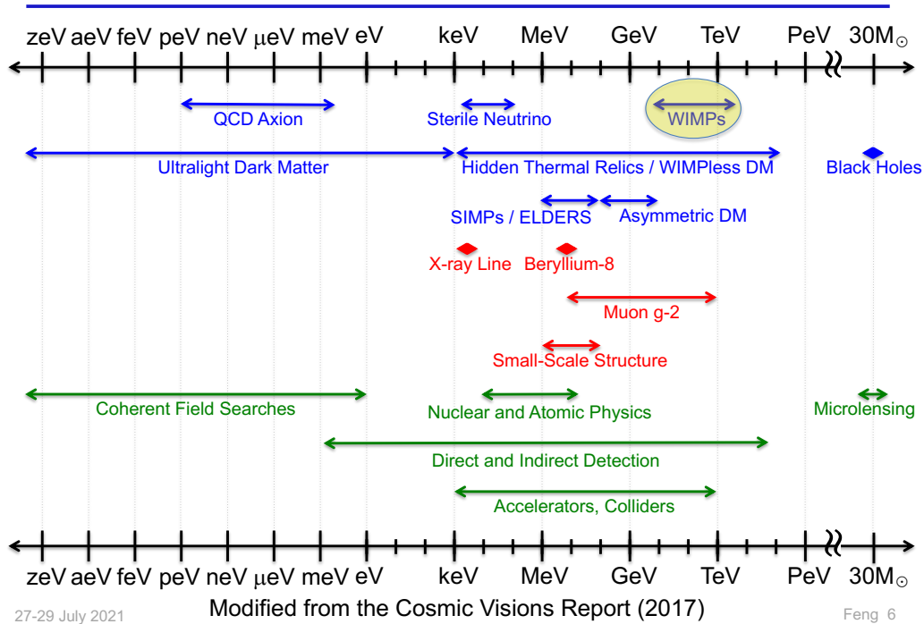
Figure 2: The landscape of particle dark matter candidates (blue), spanning almost a 100 orders of magnitude in mass, along with interesting anomalies (red) and detection methods (green). WIMPs are highlighted.
