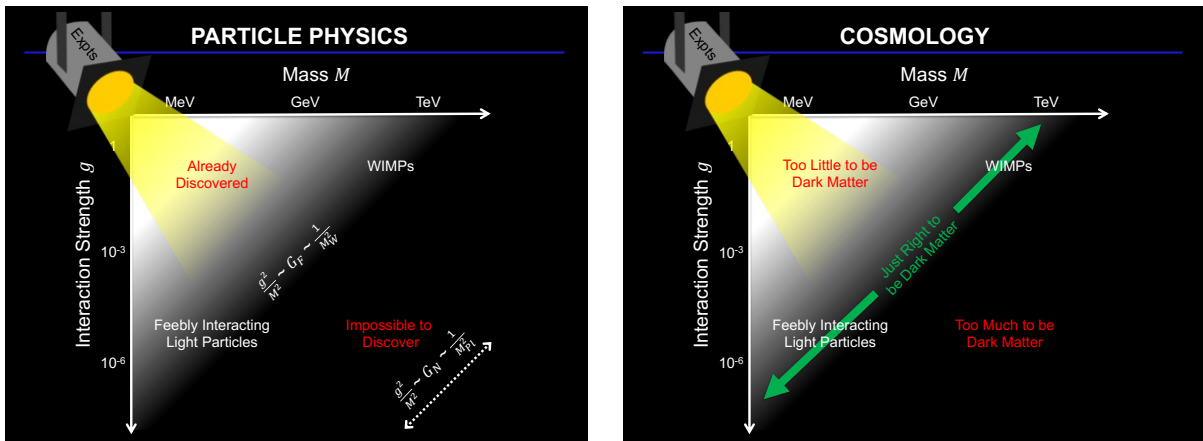
Figure 3: The new particle landscape in the (mass, coupling) plane from the perspectives of particle physics (left) and cosmology (right). On the left, WIMPs lie on the diagonal with g^2/M^2 \sim G_F , the Fermi constant, where many particle theories predict new particles, and which is also the current frontier of particle experiments. On the right, WIMPs lie on the same diagonal where particles are produced in thermal freezeout with the correct relic density to be dark matter. The triple coincidence of motivations from particle theory, particle experiment, and cosmology is known as the WIMP miracle.
