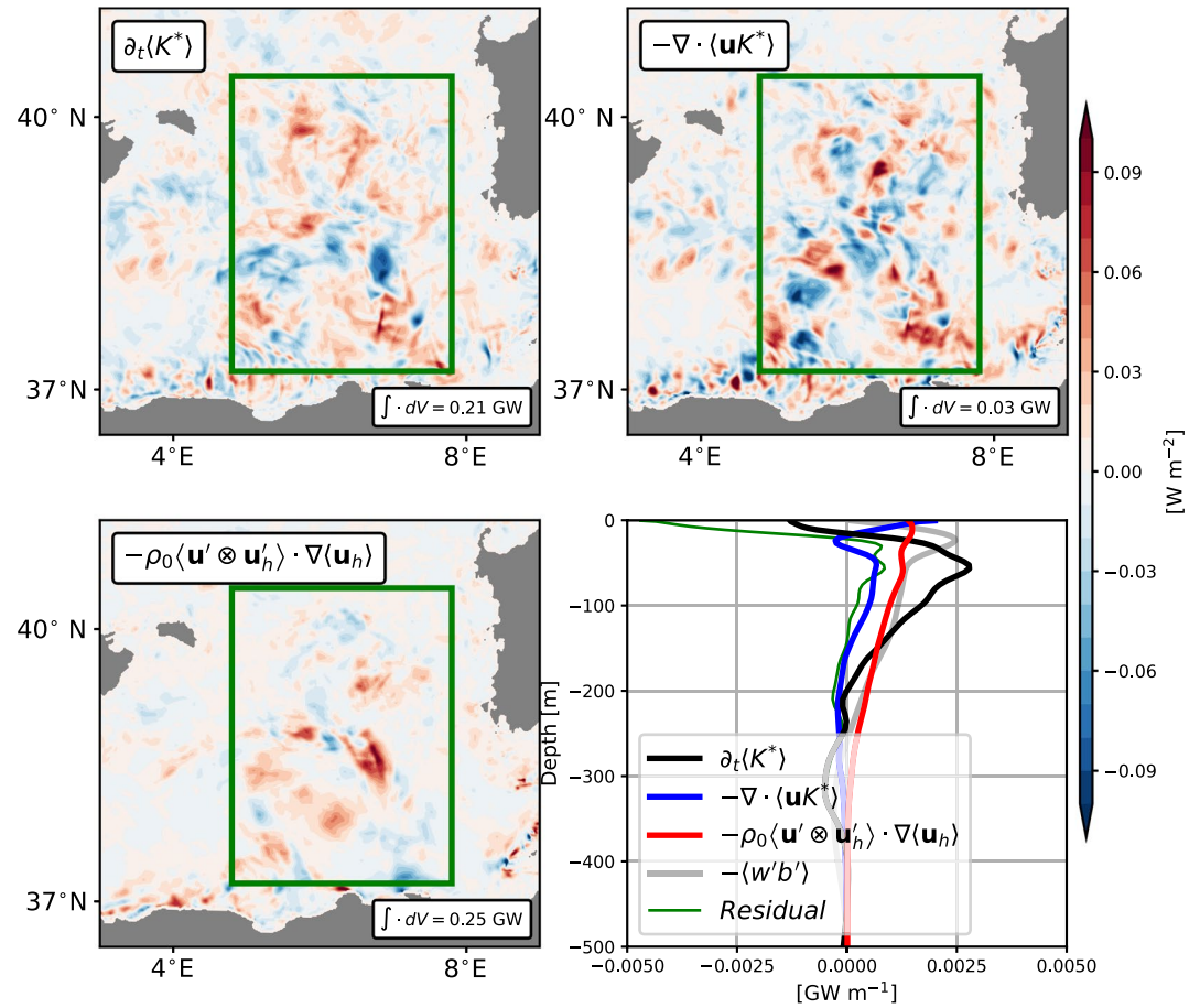
Figure 4. Same as Figure 3, but for the IKE budget. The advection of IKE (upper right panel) includes advection by both the mean flow ( -\nabla \cdot \langle \mathbf{u} \rangle \langle K^* \rangle ) and the turbulent flow ( -\nabla \cdot \langle \mathbf{u}' K^* \rangle ). Turbulent potential to kinetic energy conversion rate ( -\langle w'b' \rangle ) is also shown in gray and its net contribution within the green box is of about +0.20 GW. Note the change in amplitude of the colorbar as compared to Figure 3.
