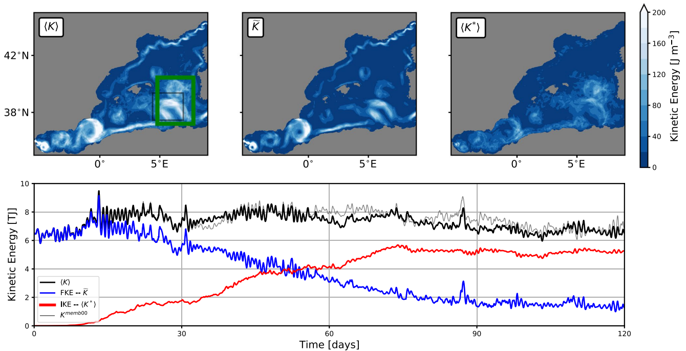
Figure 2. (Upper panels) Spatial maps of surface currents ensemble mean kinetic energy of the full flow ( \langle K \rangle ; left), kinetic energy of the ensemble mean flow ( \langle \tilde{K} \rangle , FKE; center) and the ensemble mean kinetic energy of the turbulent flow ( \langle K^* \rangle , IKE; right) after 60 days of simulation. (Lower panel) 120-day long time series of these quantities, integrated within the green box. The time series of the kinetic energy of a given member is provided for reference (gray line). Units of the spatial maps are \text{J m}^{-3} and those of the time series are terrajoules (1 TJ = 10^{12} J). The black box on top left panel is used to validate our recomputation of kinetic energy budgets (cf., Appendix A).
