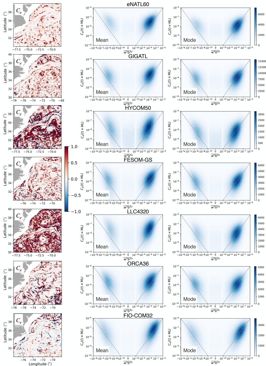
Figure E1. Snapshot of the efficiency coefficient C_e(t, x, y) diagnosed on 1 February from each simulation (left column). The joint histogram of \langle w^s b^s z \rangle and C_e(t) \times \text{MLI} during the months of February to April (right columns). The middle column shows the histogram when C_e(t) is taken as the spatial mean of C_e(t, x, y) and the right column as the spatial mode of C_e(t, x, y) . The one-to-one line is shown as the grey dashed line.
