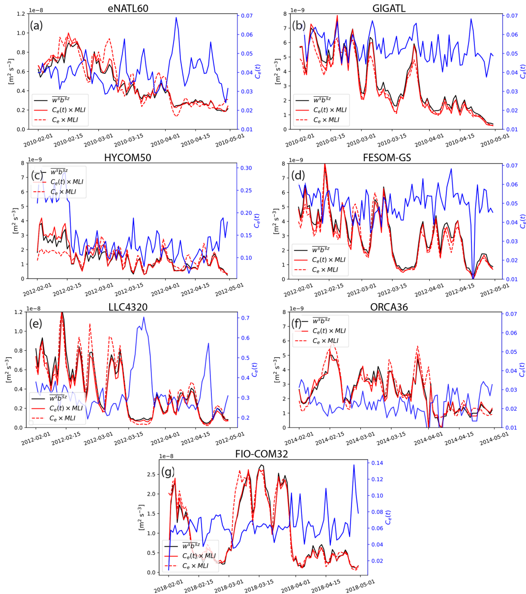
Figure 6. Time series of the spatial median of the submesoscale vertical buoyancy flux averaged over the MLD ( \langle w^s b^{s^z} \rangle ; black solid curve) and its prediction from the MLI parametrization during the months of February to April. Note that the y axes vary depending on the magnitude diagnosed from each simulation in order to highlight its temporal variability. The prediction with temporally varying C_e(t) is shown in red solid curves and with a temporally averaged (constant) C_e in red dashed curves. C_e(t) is plotted against the right y axes in blue. Three-dimensional data were not available for HYCOM25.
