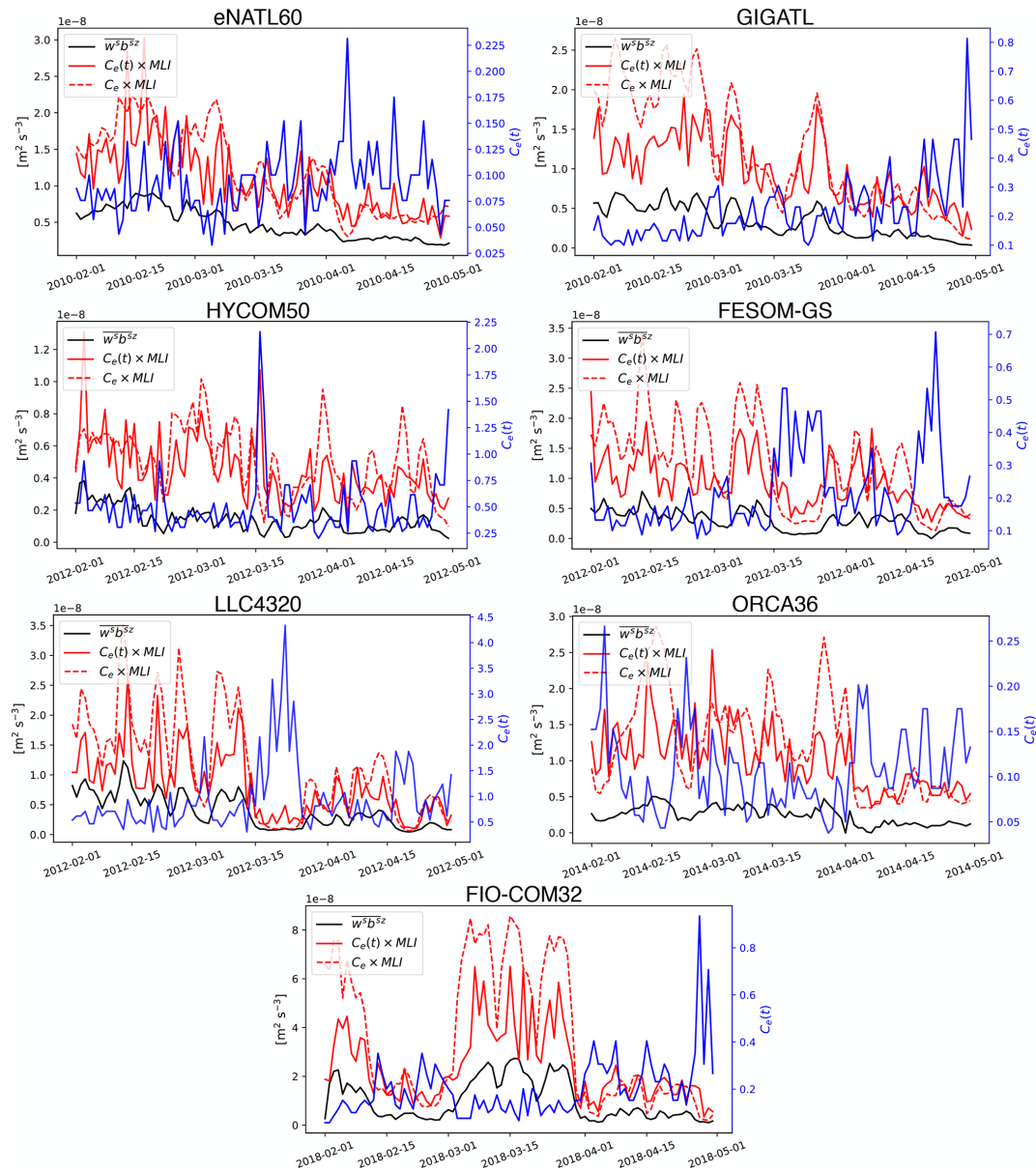
Figure E2. Time series of the spatial median of the submesoscale vertical buoyancy flux averaged over the MLD ( \overline{w^s b^s z} ; black solid curve) and its prediction from the MLI parametrization during the months of February to April, where C_e(t) is taken as the spatial mode of C_e(t, x, y) . Note that the y axes vary depending on the magnitude diagnosed from each simulation in order to highlight its temporal variability. The prediction with temporally varying C_e(t) is shown in red solid curves and with a temporally averaged (constant) C_e in red dashed curves. C_e(t) is plotted against the right-hand-side y axes in blue.
