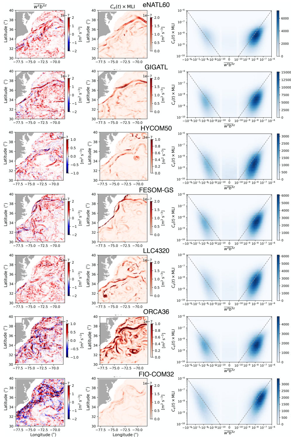
Figure 7. Snapshot of \overline{w^s b^{sz}} (left column) and C_e(t) \times \text{MLI} (middle column) on 1 February for each model. Note that the range of the color bar differs depending on the magnitude diagnosed from each model to highlight their spatial features and comparison between the submesoscale buoyancy flux and its equivalent predicted from the parametrization per simulation. Regions with bathymetry shallower than 100 m are masked out. The right column for each model shows the joint histogram of the two during the months of February to April, and the one-to-one line is shown as the grey dashed line. The histograms were computed using the xhistogram Python package (Abernathy et al., 2021c).
