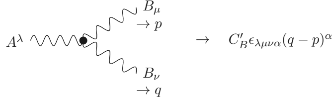
Figure 6. Feynman amplitude for Wess–Zumino term in eq. (C.12).
