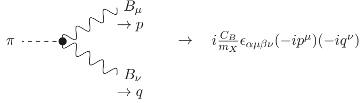
Figure 5. Example diagram from dimension-5 counterterms in last line of eq. (C.1) model.
