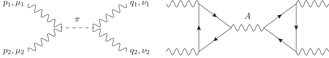
Figure 4. Z\gamma \rightarrow Z\gamma scattering through an s -channel \pi (left) or A (right, with 3 cross diagrams not pictured).
