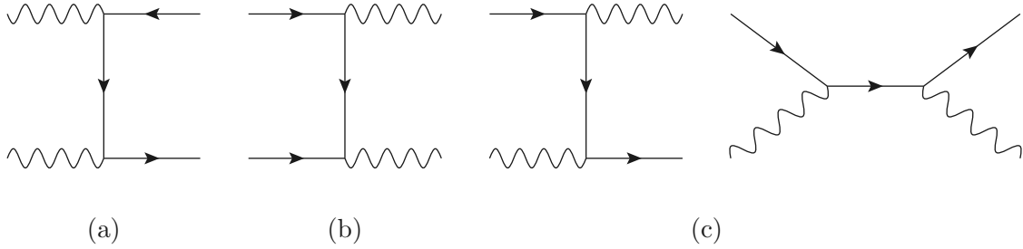
Figure 1. Diagrams for 2-2 scattering amplitudes with two fermions and two gauge bosons: (a) XX \rightarrow f\bar{f} ; (b) f\bar{f} \rightarrow XX ; (c) fX \rightarrow fX . [We have omitted the u -channel diagrams for (a), (b).] When \partial_\mu j_A^\mu \neq 0 due to the explicit violation of the global axial current by the fermion mass, the amplitudes for the longitudinally-polarized X field grow with energy proportional to m_f \sqrt{s}/m_X^2 .
