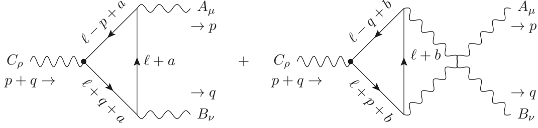
Figure 2. Triangle diagrams responsible for the coupling of A^\mu (decomposed from X^\mu = A^\mu - \partial^\mu \pi / m_X ) to two gauge bosons B^\nu and C^\rho . We have labeled Lorentz indices and directions of four-momenta according to their use in the main text.
