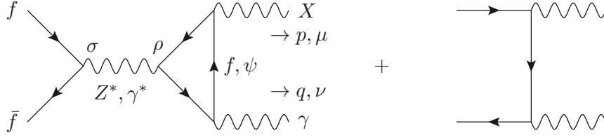
Figure 3. Diagrams for f\bar{f} \rightarrow X\gamma , with f an SM fermion: if only anomalous \psi couple to X , only the left diagram is relevant; otherwise, if f also couples to X , there are the t - and u -channel diagrams as well (cross diagrams not shown).
