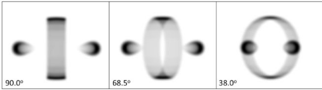
Figure 4. Type (E) shell of Fig. 3 for fitting geometry at 90^\circ and the best-fitting inclinations for the observed spectral lines, i.e. 68.5^\circ and 38.0^\circ .
