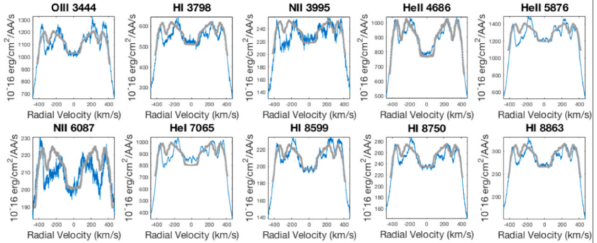
Figure 6. Unblended lines with SHAPE fit at 68.5^\circ inclination (SHAPE model overlaid in grey; Figs 4 and 5).
