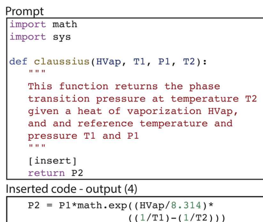
Fig. 2 Example prompt and code generated for the database example 'clausius'. Full output is the prompt with '[insert]' replaced by code in the lower box. Davinci passed our automated check for this example on three out of five tries.
