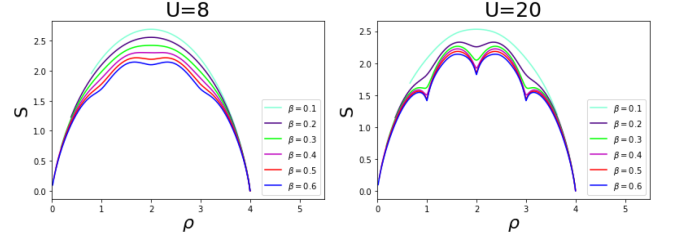
FIG. 4: Entropy as a function of density for several values of \beta and U/t = 8 and 20 . As the system enters the strongly correlated regime sharp cusps develop at integer densities.
