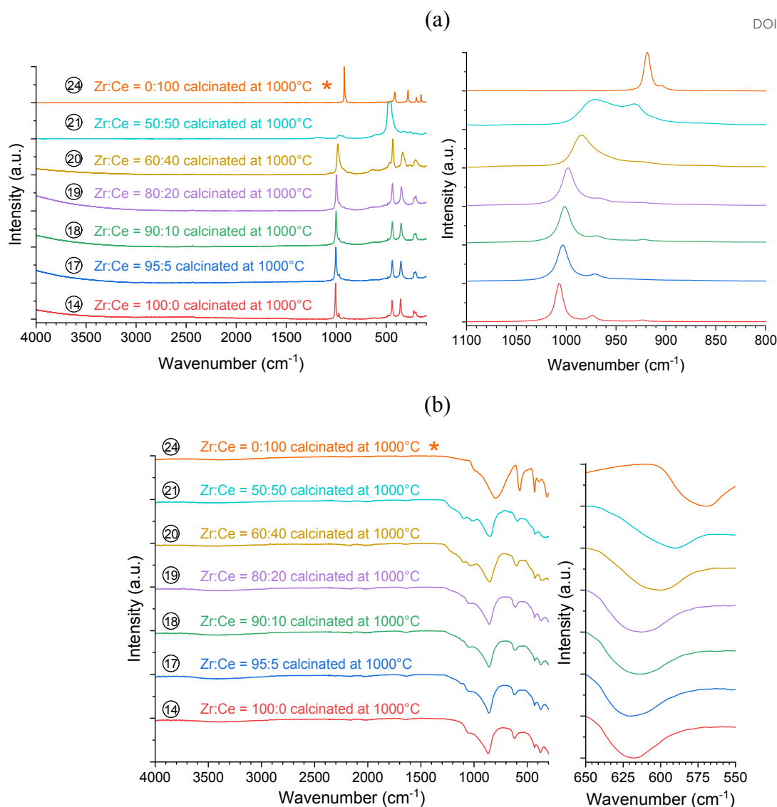
Figure 13. Raman (a) and IR (b) spectra recorded for annealed (\text{Zr,Ce})\text{SiO}_4 solid solutions with \text{Zr:Ce} = 100:0 (14), \text{Zr:Ce} = 95:5 (17), \text{Zr:Ce} = 90:10 (18), \text{Zr:Ce} = 80:20 (19), \text{Zr:Ce} = 60:40 (20), \text{Zr:Ce} = 50:50 (21) prepared under hydrothermal conditions ( T = 250^\circ\text{C} , 7 days, \text{pH} = 1.0 ) starting with \text{Zr} + \text{Ce} and silicate concentrations of 0.2 \text{ mol}\cdot\text{L}^{-1} . * Reference \text{CeSiO}_4 sample ( T = 150^\circ\text{C} , 7 days, \text{pH} = 6.5 ) starting with cerium and silicate concentrations of 0.2 \text{ mol}\cdot\text{L}^{-1} (24).
