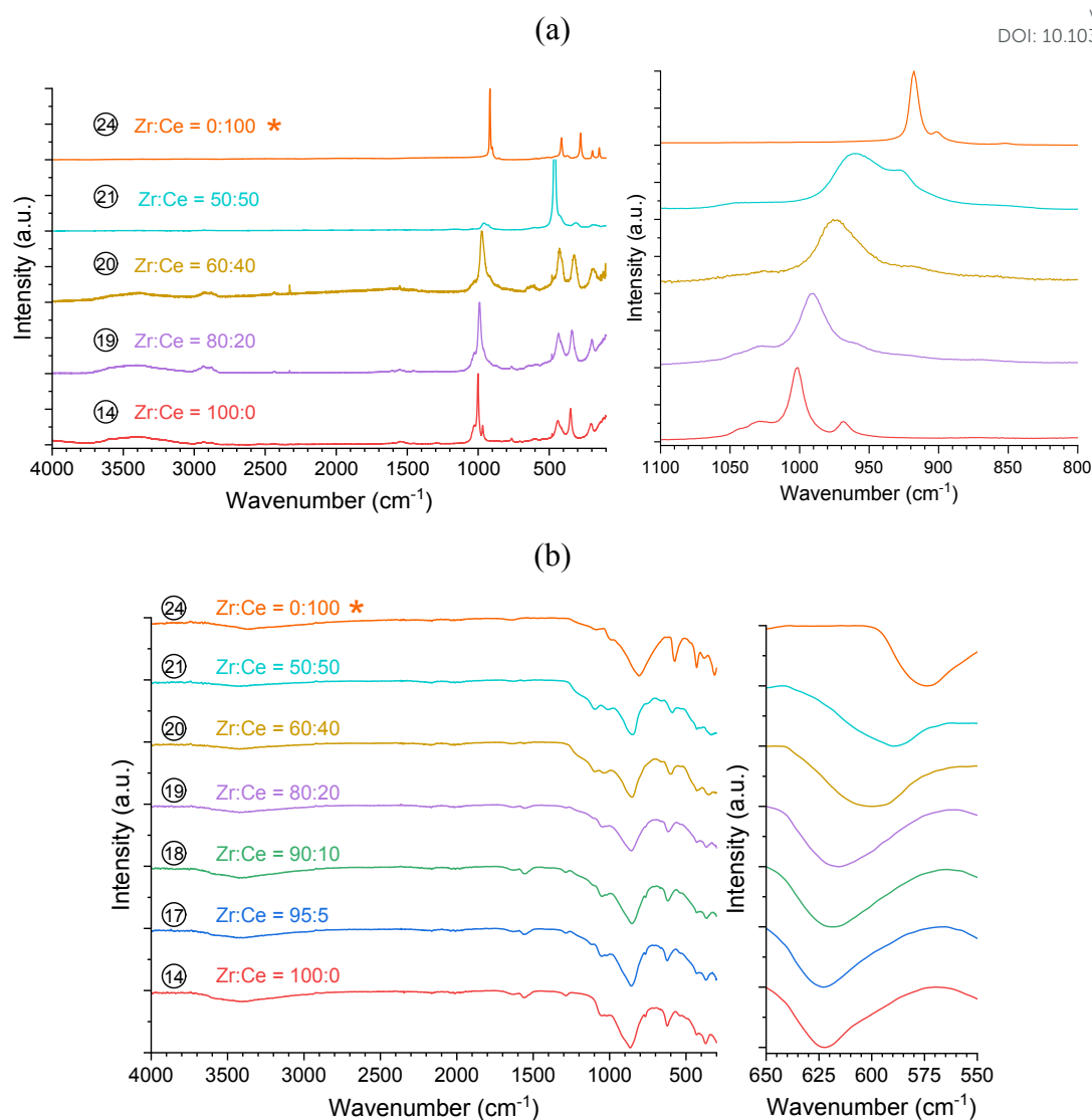
Figure 12. Raman (a) and IR (b) spectra recorded for pristine (\text{Zr,Ce})\text{SiO}_4 solid solutions with Zr:Ce = 100:0 (14), Zr:Ce = 95:5 (17), Zr:Ce = 90:10 (18), Zr:Ce = 80:20 (19), Zr:Ce = 60:40 (20), Zr:Ce = 50:50 (21) prepared under hydrothermal conditions ( T = 250^\circ\text{C} , 7 days, \text{pH} = 1.0 ) starting with Zr + Ce and silicate concentrations of 0.2 \text{ mol}\cdot\text{L}^{-1} . * Reference \text{CeSiO}_4 sample ( T = 150^\circ\text{C} , 7 days, \text{pH} = 6.5 ) starting with cerium and silicate concentrations of 0.2 \text{ mol}\cdot\text{L}^{-1} (24).
