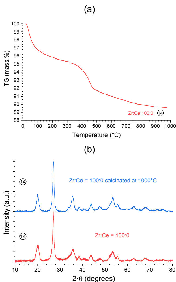
Figure 7. TGA analysis (a) and PXRD patterns (b) recorded for a pristine and annealed (after TGA, 1000^\circ\text{C} ) \text{ZrSiO}_4 sample (14) prepared under hydrothermal conditions ( T = 250^\circ\text{C} , 7 days) at \text{pH} = 1.0 starting with zirconium and silicate concentrations of 0.2 \text{ mol}\cdot\text{L}^{-1} .
