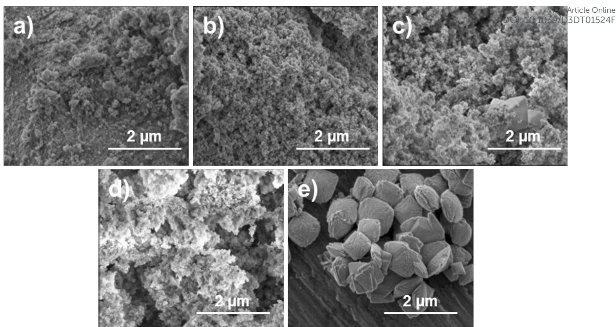
Figure 16. SEM micrographs recorded for (\text{Zr,Ce})\text{SiO}_4 solid solutions with a) \text{Zr:Ce} = 100:0 (14), b) \text{Zr:Ce} = 60:40 (20), c) \text{Zr:Ce} = 50:50 (21), d) \text{Zr:Ce} = 30:70 (23) prepared under hydrothermal conditions ( T = 250^\circ\text{C} , 7 days, \text{pH} = 1.0 ) starting with \text{Zr} + \text{Ce} and silicate concentrations of 0.2 \text{ mol}\cdot\text{L}^{-1} . e) Reference \text{CeSiO}_4 sample ( T = 150^\circ\text{C} , 7 days, \text{pH} = 6.5 ) starting with cerium and silicate concentrations of 0.2 \text{ mol}\cdot\text{L}^{-1} (24).
