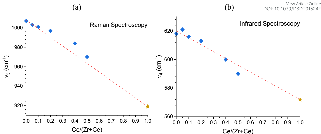
Figure 14. Variation of the \nu_3 (a) and \nu_4 (b) observed by Raman and IR spectroscopy for (\text{Zr,Ce})\text{SiO}_4 (annealed samples at 1000°C) versus the expected chemical composition. * Reference \text{CeSiO}_4 sample wasn't obtained in the same chemical conditions as the (\text{Zr,Ce})\text{SiO}_4 samples. Errors bars are smaller than the data point size ( \pm 1 \text{ cm}^{-1} ).
