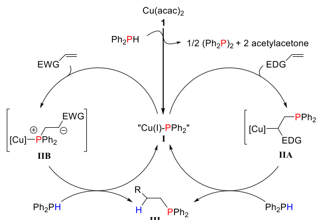
Scheme 2. Proposed mechanism of copper-catalyzed hydrophosphination
