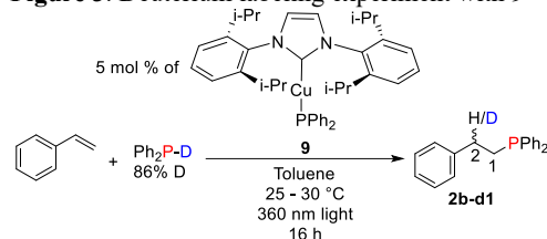
Figure 3. Deuterium labeling experiment with 9
