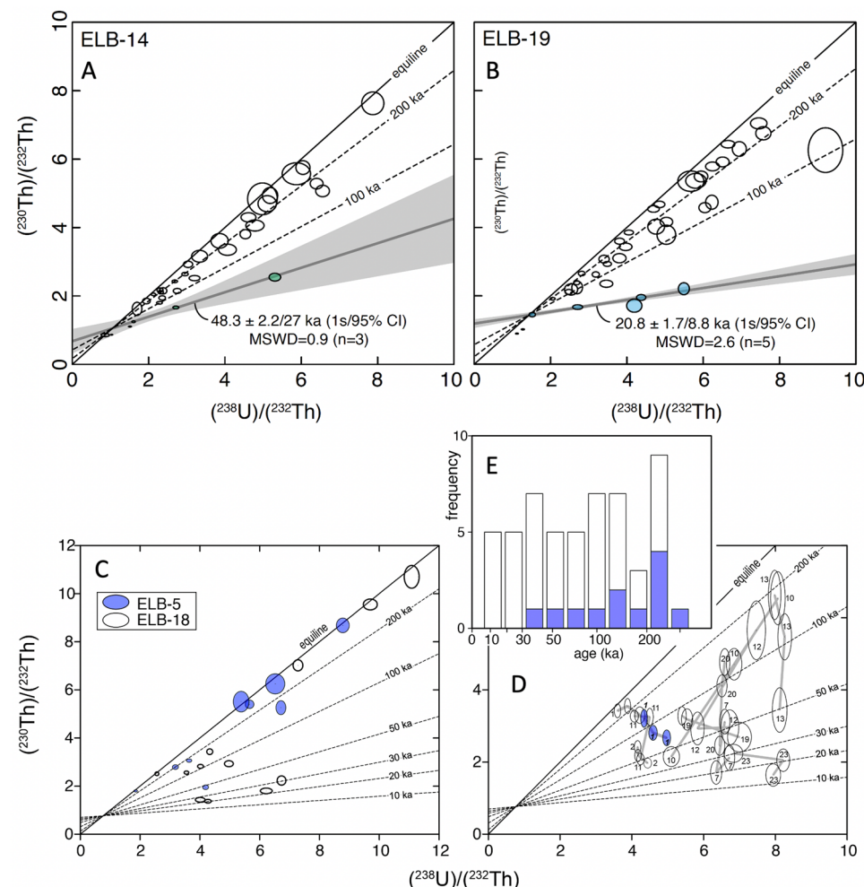
Figure 3. Results of U–Th dating of zircon cores ((A,B), by LAICPMS) and outermost rims ((C–E), depth profiling by SIMS). Notice significant inheritance of older zircons. In (C), average ages, where no significant age variability was detected with depth ( \sim 3 \mu\text{m} total depth profile); (D) ages calculated for \sim 1 \mu\text{m} outermost rim penetration in Holocene lavas, see Methods for further explanation. Numbers next to error ellipses (displayed at 1 s uncertainty) correspond to zircon number; gray lines connect progressively deeper zircon layers in each profile. (E) Histogram of all model ages of dated zircon rim indicating protracted zircon crystallization even for the outermost 1–3 \mu\text{m} of individual zircon crystals ranging between 13.9 ka and secular equilibrium (> 300 ka). Model ages are displayed for an initial (^{230}\text{Th})/(^{232}\text{Th}) corresponding to whole rock Th and U abundances, assuming secular equilibrium. The younger isochron age in A and B is based on the youngest zircon cores, but these are \sim 20 to 37 kyr older than the presumed Late Holocene eruption age of these lavas, as is the zircon surface age in (D), suggesting that zircons were dissolving prior to the eruption (see Fig. S1).
