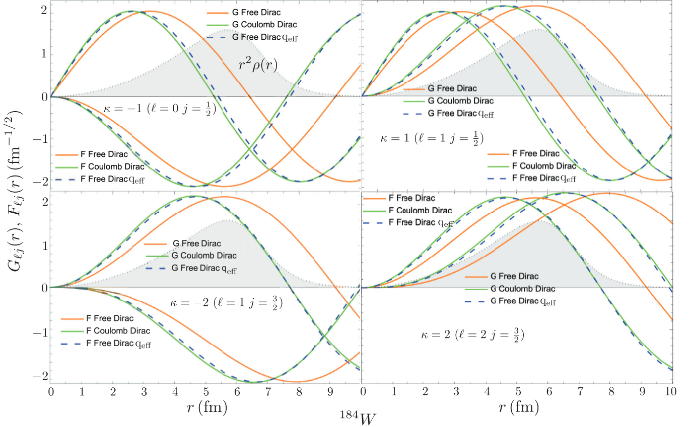
FIG. 3. As in Fig. 2 but for ^{184}\text{W} .
