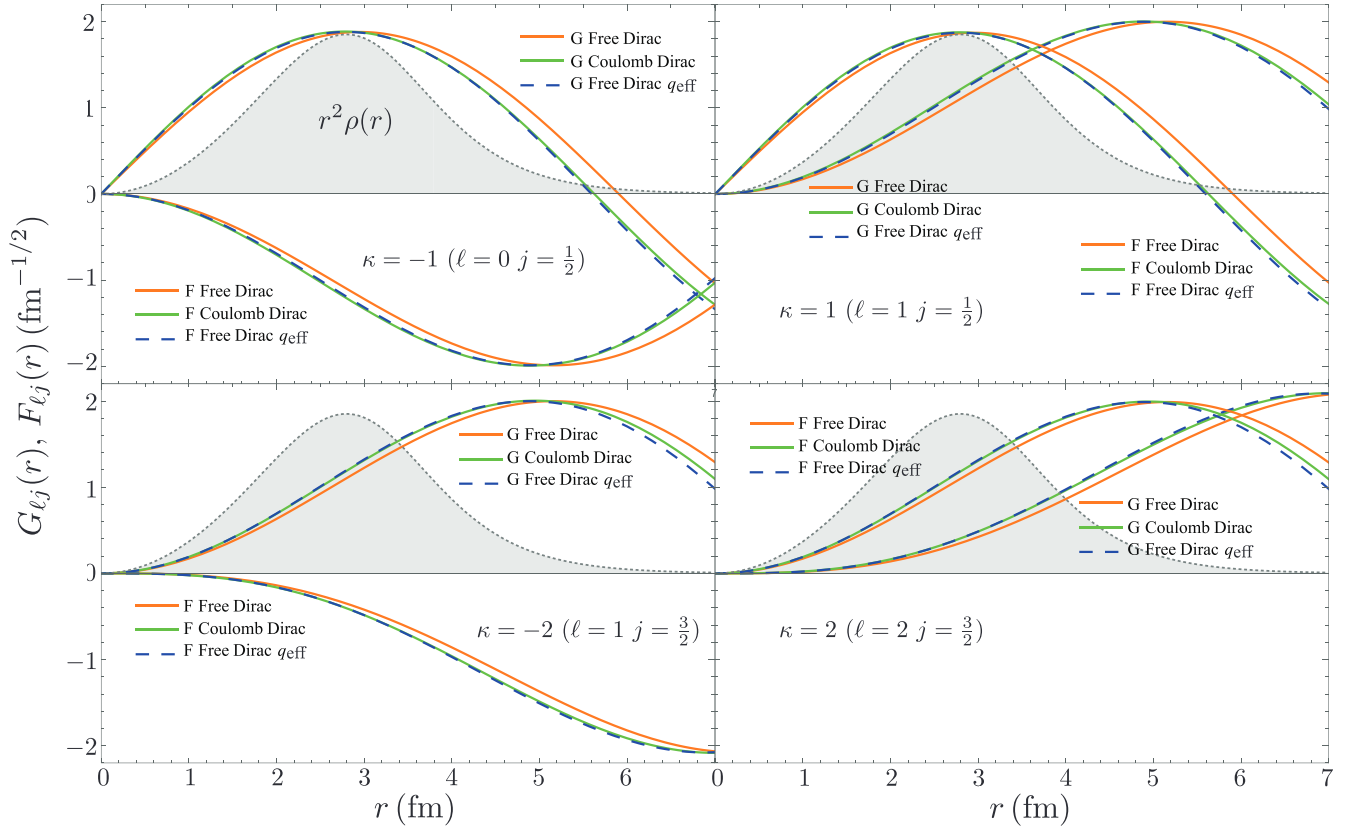
FIG. 2. The Dirac Coulomb solutions G(r) and F(r) for the highly relativistic outgoing electron produced in \mu^- \rightarrow e conversion in ^{27}\text{Al} (green line) are compared to the free solution (orange) and to the free solution evaluated with q_{\text{eff}} (blue dashed), for low partial waves. The nuclear charge distribution is shown by the shading (arbitrary normalization). The agreement between the Coulomb and free solutions evaluated with q_{\text{eff}} is quite good.
