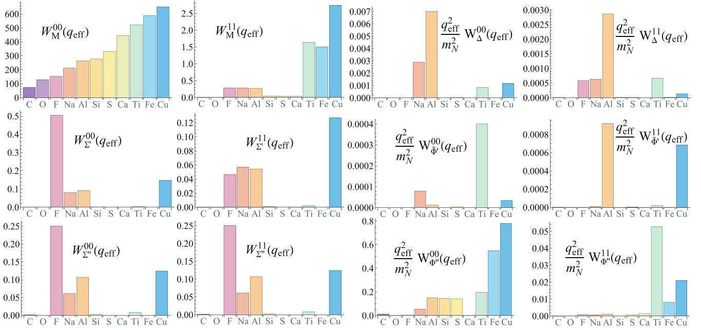
FIG. 8. The nuclear responses to both allowed (left two panels) and velocity-induced (right) operators, for the 11 targets considered in this paper. Target properties can significantly alter operator responses, providing an important diagnostic tool for determining the source of CLFV, should it be observed.
