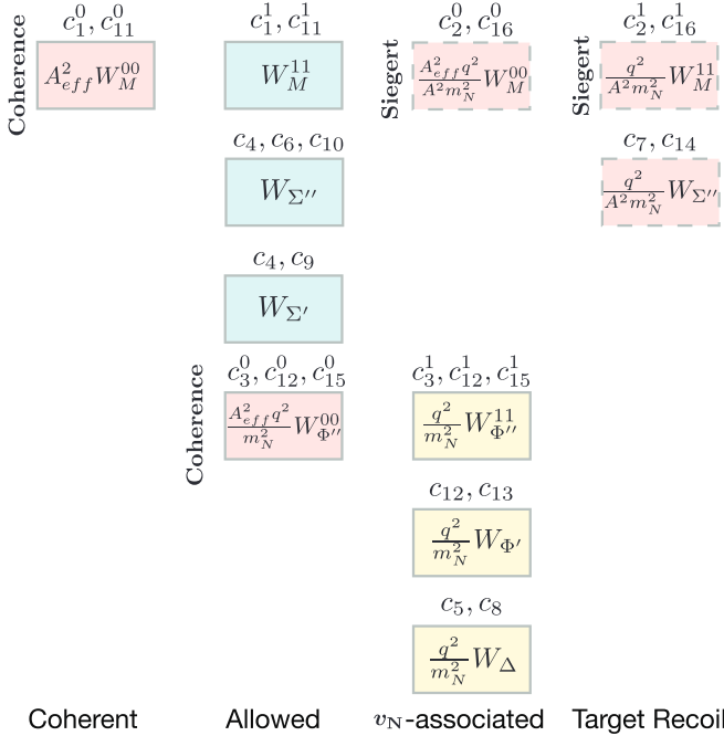
FIG. 9. Nuclear- vs nucleon-level NRET, with strong operators to the left and weak ones to the right. Naïvely, NRET operators are either allowed (blue-green) or velocity suppressed (yellow). The nucleus alters this pattern, as indicated in pink. Distinct forms of nuclear coherence enhance the responses W_M^{00} and W_{\Phi''}^{00} by factors typically \approx 100 in ^{27}\text{Al} . Other nucleon-level NRET operators, O_2 , O_7 , O_{14} , and O_{16} , are forbidden by selection rules or current conservation, apart from small nuclear recoil effects, suppressing these operators by \approx \frac{1}{100} .
