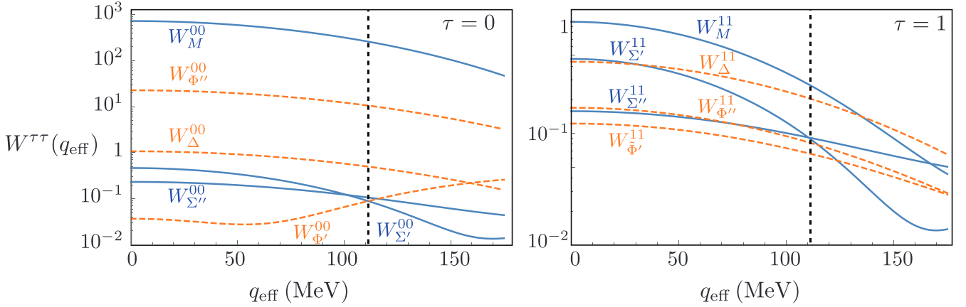
FIG. 6. The nuclear response functions for the six operators contributing to elastic \mu \rightarrow e conversion on ^{27}\text{Al} . Here W_{OO}^{\tau\tau}(q_{\text{eff}}) denotes W_{OO}^{\tau\tau}(q_{\text{eff}}) . The left (right) panel gives the results for isoscalar (isovector) coupling. The response functions are needed at the q_{\text{eff}} indicated by the dashed line. The results in blue correspond to charge and spin couplings, while those in orange correspond to the velocity-dependent operators where the response functions are accompanied by the additional factor q_{\text{eff}}^2/m_N^2 \approx 0.014 .
