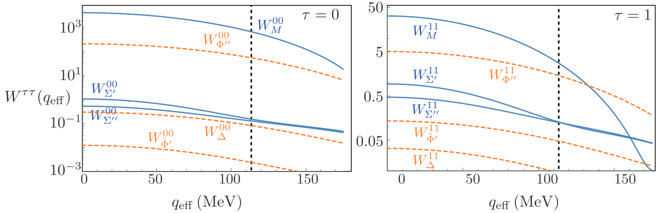
FIG. 7. As in Fig. 6 but for Cu.
