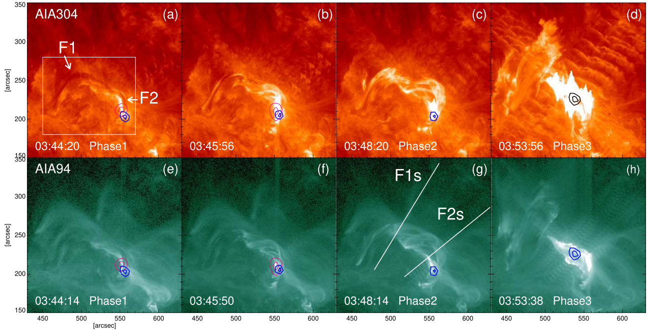
Figure 2. Time sequence of AIA 304 Å (top) and 94 Å (bottom) images. Panels (a) and (e) show the onset of Phase 1, panels (b) and (f) capture the peak of Phase 1, while panels (c), (g), and (d), (h) represent Phase 2 and Phase 3, respectively. The blue and red contours are NoRH 17 GHz and RHESSI 20–40 keV measurements, respectively. The contour levels are plotted at 70% and 90% of their maximum intensity. The line segments in panel (g) indicate directions of the eruption of filaments F1 and F2 and they also represent slits used to produce time-space plots shown in Figure 3. A color version of this figure is available in the online journal.
