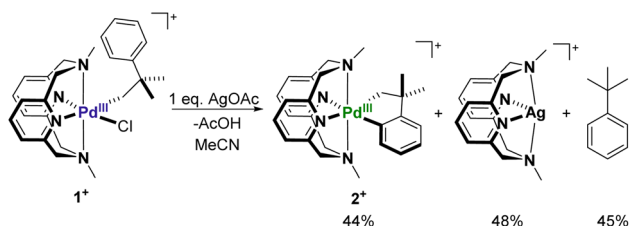
Scheme 2 C–H activation at 1^+ in the presence of \text{AgOAc} .
