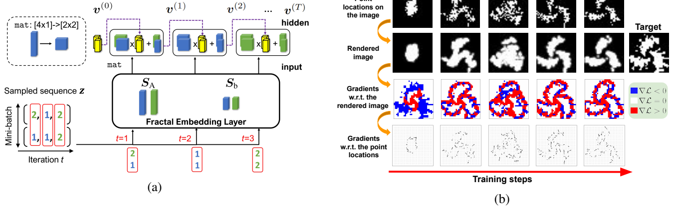
Figure 2: (a) Fractal embedding layer in subsection 6. We show a case of T = 3 and batch size = 2. The purple dashed lines indicate the point transition (like the hidden vector in RNNs). (b) Differentiable rendering in subsection 6. We show that the gradients w.r.t. the rendered image can be translated into 2D gradient vectors w.r.t. the IFS points, i.e., \nabla_{v^{(t)}} \mathcal{L} \in \mathbb{R}^2, \forall t \in \{1, \dots, T\} (zoom-in for better resolutions).
