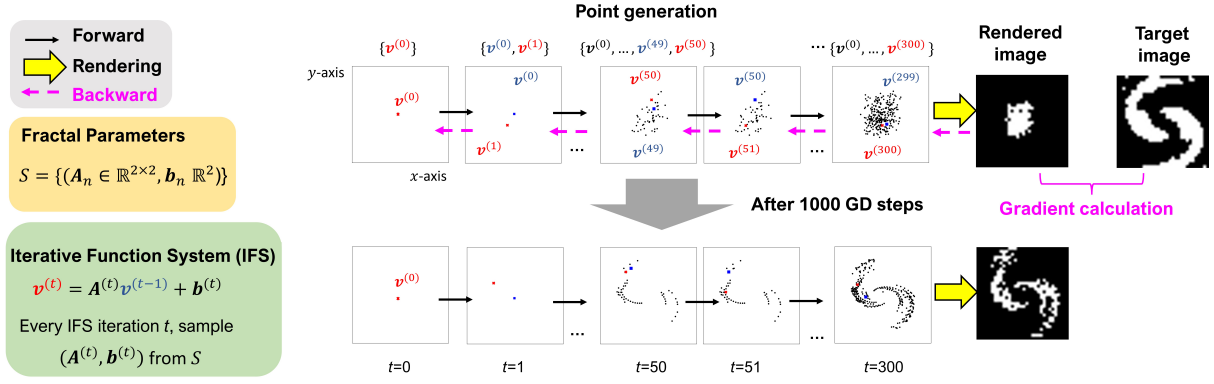
Figure 1: Overview of our approach, which aims to learn the fractal parameters \mathcal{S} so that the generated point sequence by IFS (i.e., \{v^{(0)}, \dots, v^{(300)}\} ), after being rendered onto an image, is close to the target image. We learn \mathcal{S} by gradient descent (GD). As shown, after 1000 GD steps, we can learn high-quality \mathcal{S} to generate images that are visually close to the target one.
