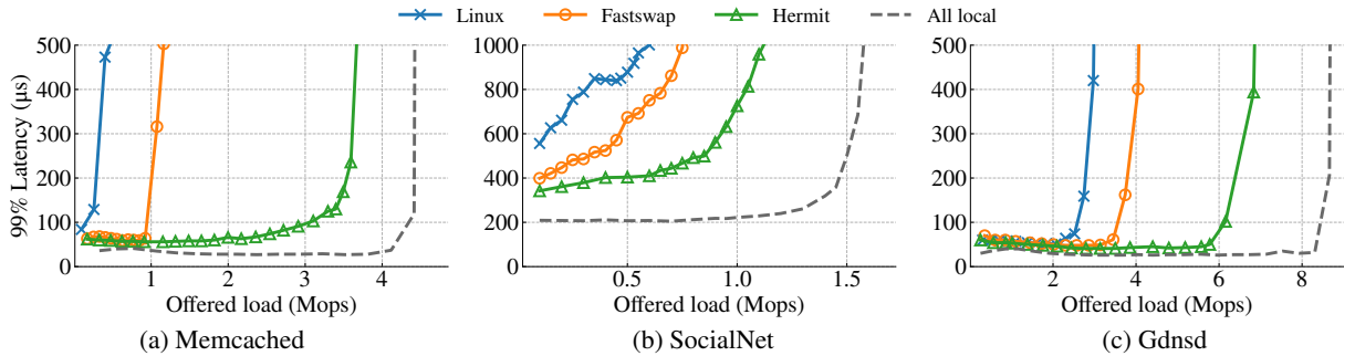
Figure 8: Hermit achieves significantly lower 99% latency than Fastswap and Linux under the same fixed local memory ratio and varying load. For Memcached and Gdnspd, Hermit achieves 99% latency close to the ideal local-only case. SocialNet is more challenging due to its higher per-request memory footprint, but Hermit still achieves 74% load capacity of the ideal case.
