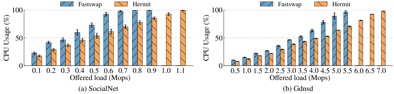
Figure 19: For SocialNet and Gdnsd, Hermit still saves 10%–40% CPU cycles under varying load compared with Fastswap, which is the key enabler it can achieve low tail latency under high load.
