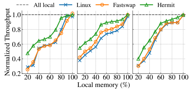
(a) Spark (68.4s) (b) XGBoost (42.2s) (c) Cassandra (72.6s) Figure 9: We measured the throughput of batch applications achieved by different swap systems normalized to the ideal local-only setup. Hermit outperforms other baselines. The number in the parenthesis shows the ideal execution time.
