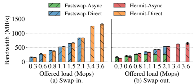
Figure 16: Hermit’s optimizations do not incur additional network usage during swap-ins/-outs compared to Fastswap.
