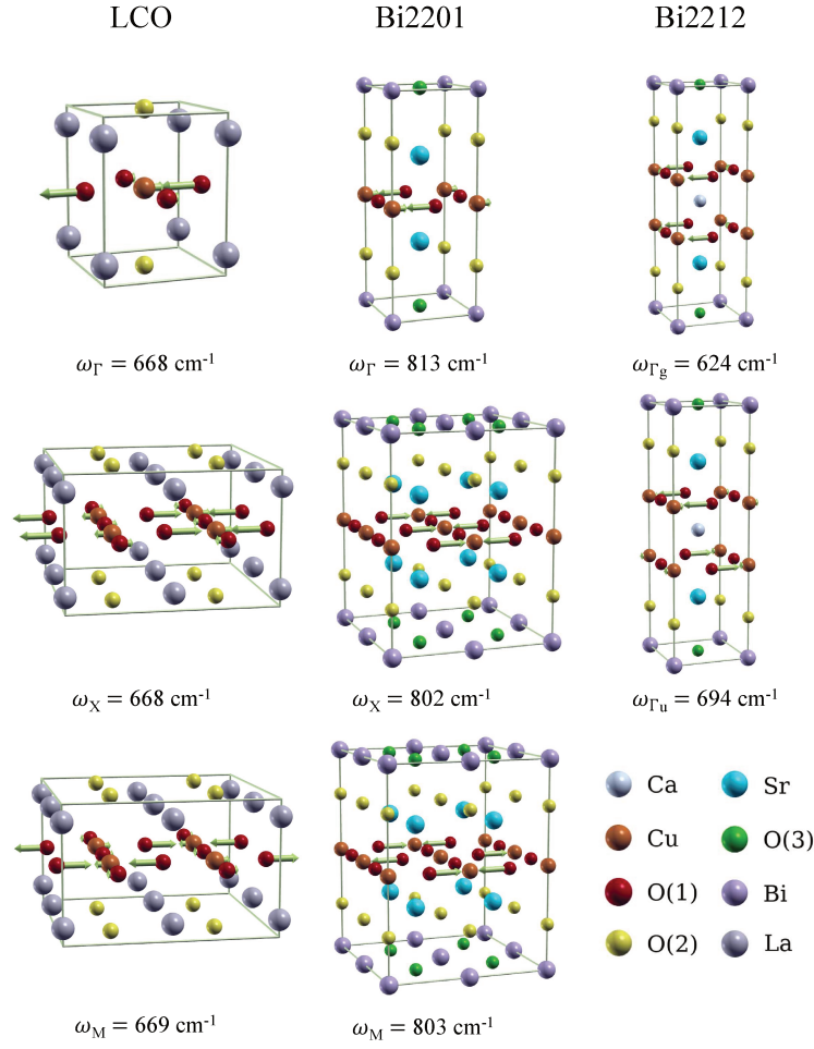
Figure 2: Cu-O bond stretching modes for \text{La}_2\text{CuO}_4 (LCO), \text{Bi}_2\text{Sr}_2\text{CuO}_6 (Bi2201) and \text{Bi}_2\text{Sr}_2\text{CaCu}_2\text{O}_8 (Bi2212) at the \Gamma , X and M points in the Brillouin zone ( \Gamma -only for Bi2212).
