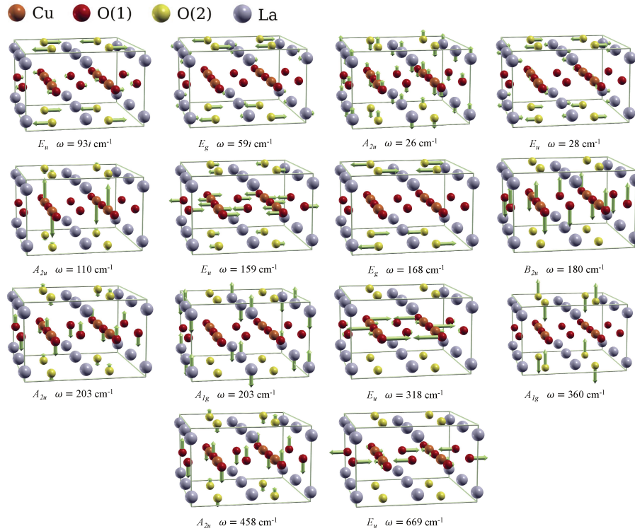
Figure A3: All LCO modes at the M point, represented in a 2 \times 2 supercell.
