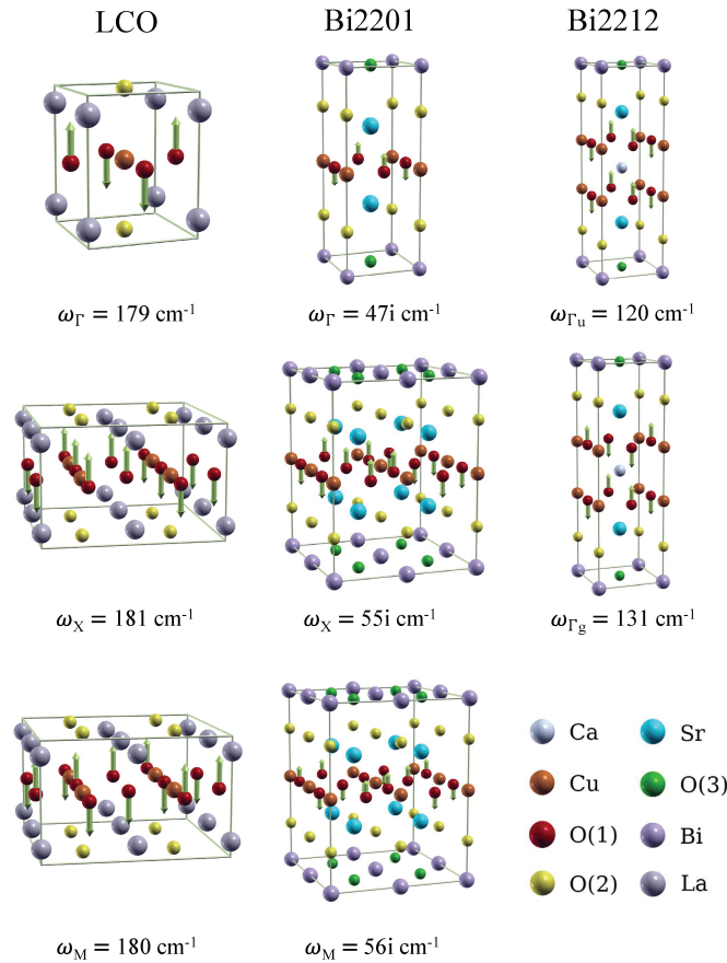
Figure 1: Cu-O bond buckling modes for \text{La}_2\text{CuO}_4 (LCO), \text{Bi}_2\text{Sr}_2\text{CuO}_6 (Bi2201) and \text{Bi}_2\text{Sr}_2\text{CaCu}_2\text{O}_8 (Bi2212) at the \Gamma , X and M points in the Brillouin zone ( \Gamma -only for Bi2212). Note that the buckling modes for Bi2201 frequencies are imaginary at all three points, indicating a structural instability across the Brillouin zone.
