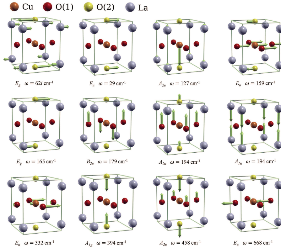
Figure A1: All optical LCO modes at the \Gamma point.
