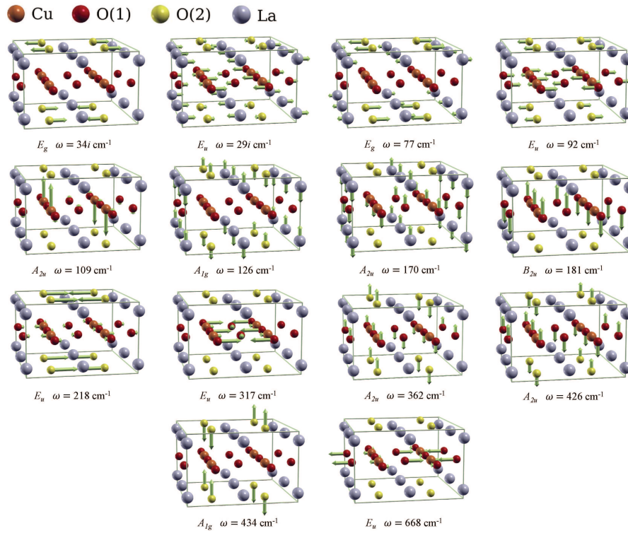
Figure A2: All LCO modes at the X point, represented in a 2x2 supercell.
