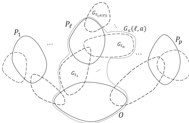
Fig. 3 An example of G_{\leq}(\ell, a) . Here the regions enclosed by dashed lines represent V(G_{t'}) , where t' runs over \mathcal{A}(\ell) . The region enclosed by the dotted line is G_{\leq}(\ell, a)
