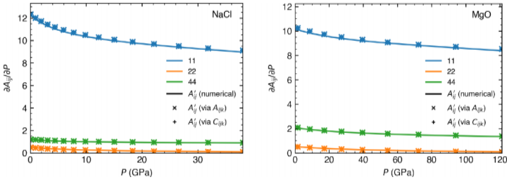
FIG. 8. Pressure derivative of SOECs vs pressure for NaCl and MgO. Curves denote numerical pressure derivatives of the elastic coefficients; \times indicates predictions based on Eq. (25); + indicates predictions based on Eq. (26).
