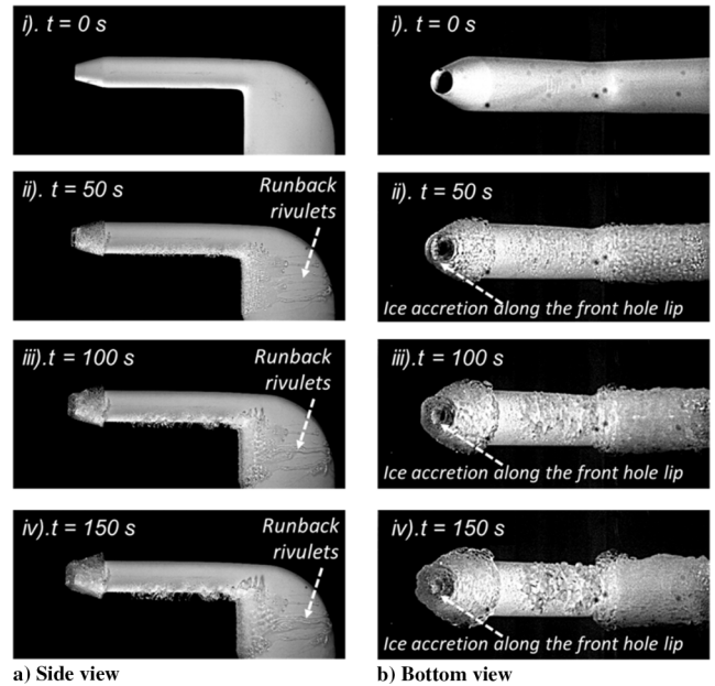
Fig. 3 Typical snapshot images to reveal the dynamic ice accretion process on the Pitot probe under the glaze icing condition of V_\infty = 40 m/s, T_\infty = -5.0^\circ\text{C} , and LWC = 2.0 g/m 3 .
