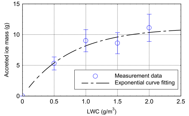
Fig. 9 The variations of the measured ice mass accreted on the Pitot probe model as a function of the LWC level of the incoming airflow at T_\infty = -5.0^\circ\text{C} .
