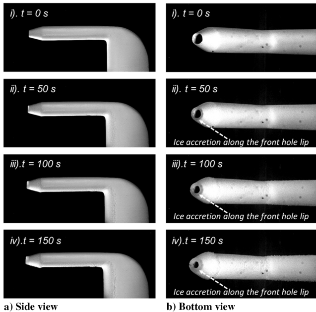
Fig. 2 Typical snapshot images to reveal the dynamic ice accretion process on the Pitot probe under the rime icing condition of V = 40 m/s, T_\infty = -15.0^\circ\text{C} , and LWC = 0.50 g/m 3 .
