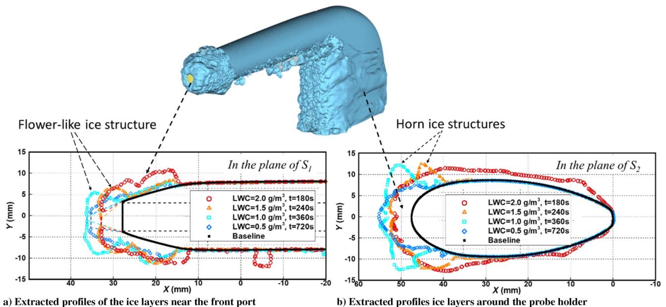
Fig. 8 Comparison of the extracted profiles of the ice layers accreted over the surface of the Pitot probe model under different test conditions.
