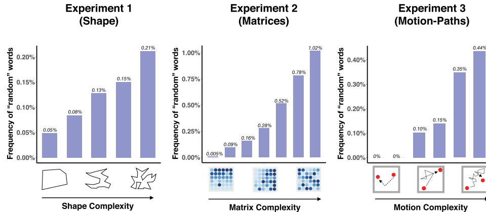
Figure 7 Results From an Analysis Exploring the Use of Words Indicating Randomness
