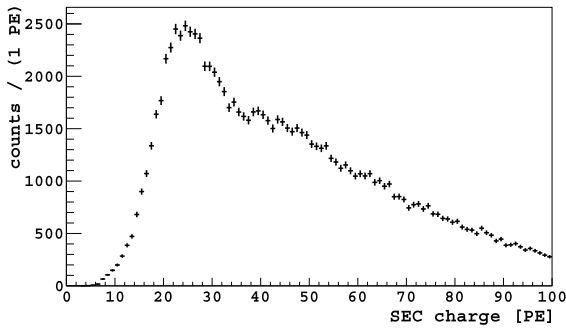
Fig. 2. SEC charge distribution for S2-echo events.
