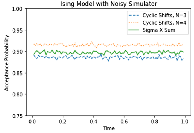
FIG. 3. Results of symmetry tests for the transverse Ising model for N = 3 and N = 4 , using IBM Quantum’s noisy simulator. The symmetries in question are given by acting simultaneously on all systems by either the cyclic group of order N or a conjugation by \delta \sigma^x \mathbf{p}^N .
