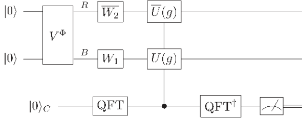
FIG. 1. Quantum circuit to test for the covariance of a unitary Hamiltonian evolution. The unitary V^\Phi generates the state j\Phi_{i_{RA}} , the maximally entangled state on RA . The evolution of the system is given by e^{-iHt} \frac{1}{2} W_1 W_2^\dagger , and the U(g) gates are controlled on a superposition over all of the elements g \in G , as in (4).
