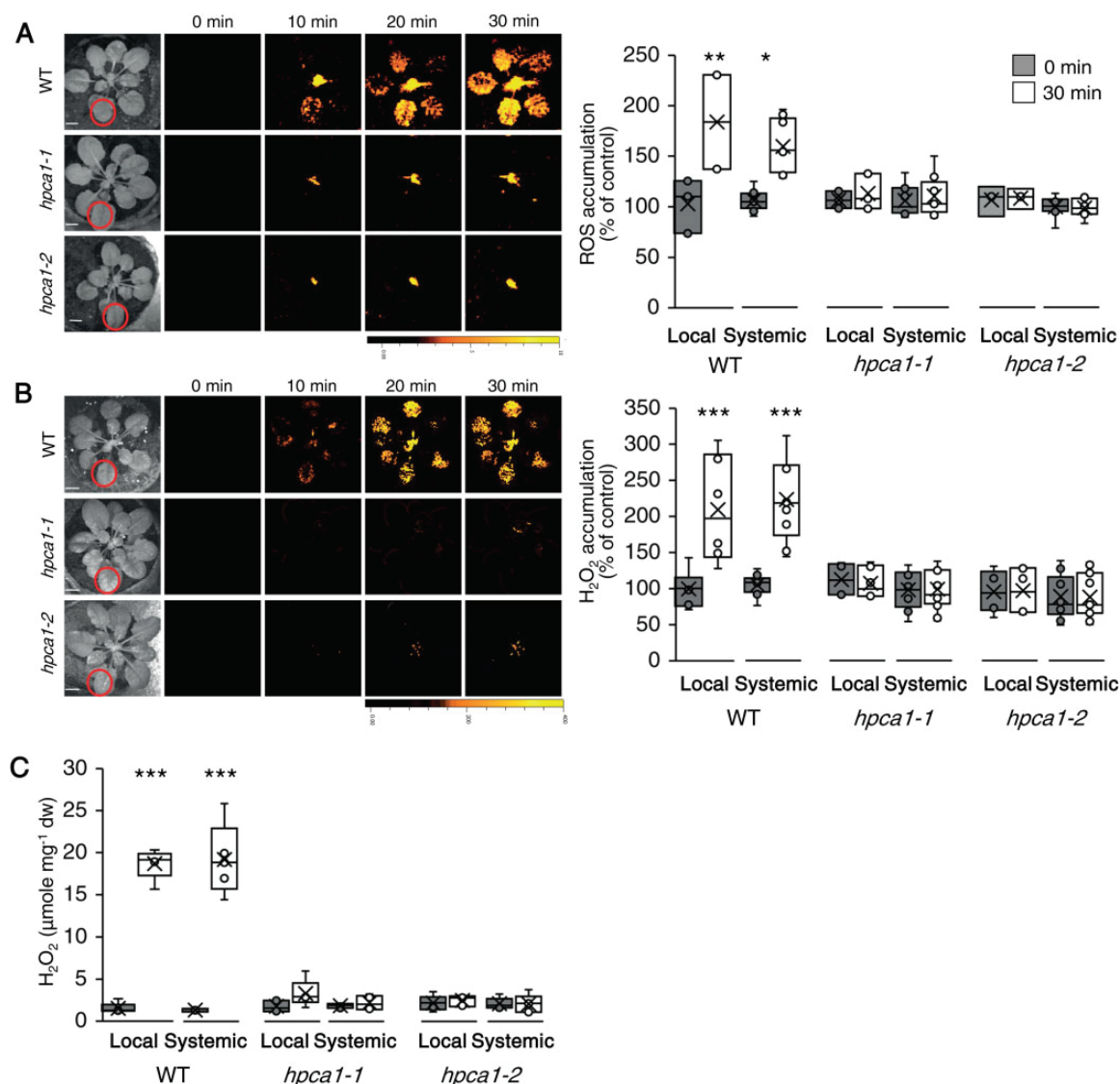
Figure 1 HPCA1 is required for systemic cell-to-cell ROS signaling in response to light stress. A, Arabidopsis plants were subjected to a HL stress treatment applied to a single leaf (Local; indicated with a circle), and ROS accumulation was imaged, using H 2 DCFDA, in whole plants (local and systemic tissues). Representative time-lapse images of whole-plant ROS accumulation in WT, hpca1-1 and hpca1-2 plants are shown alongside bar graphs of combined data from all plants used for the analysis at the 0- and 30-min time points (local and systemic). B, Same as in (A), but for whole-plant H 2 O 2 accumulation that was imaged using PO1. C, Arabidopsis plants were subjected to a HL stress treatment applied to a single leaf (Local) and the levels of H 2 O 2 were measured in extracts from local and systemic leaves using Amplex-Red. All experiments were repeated at least three times with 10 plants of each genotype per experiment. Data are presented as box plot graphs; X is mean \pm SE, N = 30 , * P < 0.05 , ** P < 0.01 , *** P < 0.001 , Student t test. Scale bar, 1 cm. See Movie 1 for live imaging.
