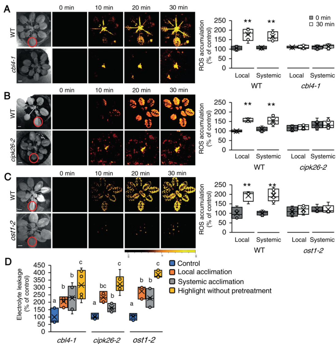
Figure 7 CBL4, CIPK26, and OST1 are required for systemic cell-to-cell ROS signaling and acclimation to light stress. A, Representative time-lapse images of whole-plant ROS accumulation in WT and cbl4-1 plants subjected to a local HL stress treatment (applied to a single local leaf; indicated with a circle) are shown alongside bar graphs of combined data from all plants used for the analysis at the 0- and 30-min time points (local and systemic). B, Same as (A), but for WT and cipk26-2 plants. C, Same as (A), but for WT and ost1-2 plants. D, Averaged measurements of leaf injury (increase in ion leakage) in WT, cbl4 , cipk26 , and ost1 plants. Measurements are shown for unstressed plants (control), local leaves subjected to a pretreatment of HL stress before a long HL stress period (local acclimation), systemic leaves of plants subjected to a local HL stress pretreatment before a long period of local HL stress was applied to a systemic leaf (systemic acclimation), and systemic leaves of plants subjected to a long HL stress period without pretreatment (HL without pretreatment). All experiments were repeated at least three times with 10 plants of each genotype per experiment. ROS accumulation was imaged using H_2DCFDA . Data are presented in (A) to (C) as box plot graphs; X is mean \pm SE, N = 30 , **P < 0.01 , Student t test. Data are presented in (D) as box plot graphs; X is mean \pm SE, N = 30 , one-way ANOVA followed by a Tukey test; lower-case letters denote significance ( P < 0.05 ). Scale bar, 1 cm.
