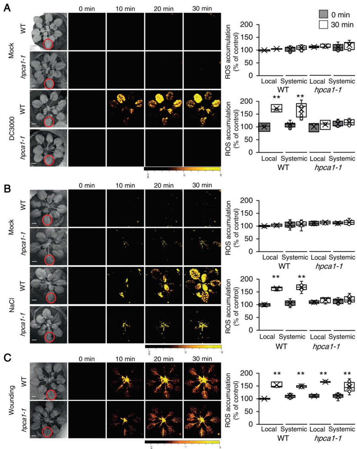
Figure 6 HPCA1 is required for systemic cell-to-cell ROS responses to bacterial infection and salt stress, but not wounding. A, Representative time-lapse images of whole-plant ROS accumulation in WT and hpca1-1 plants subjected to mock or bacterial ( Pseudomonas syringae DC3000) infection on a single local leaf are shown alongside bar graphs of combined data from all plants used for the analysis at the 0- and 30-min time points (local and systemic). B, Same as in (A), but for mock and salt stress (100-mM NaCl) applied to a single local leaf. C, Same as in (A), but for wounding applied to a single local leaf (control plants were untreated). Although the hpca1-1 mutant is deficient in cell-to-cell ROS signaling in response to salinity stress (B), it displays cell-to-cell calcium signaling in response to this stress (Supplemental Figure S3). All experiments were repeated at least three times with 10 plants of each genotype per experiment. ROS accumulation was imaged using H 2 DCFDA. Data are presented as box plot graphs; X is mean \pm SE, N = 30 , **P < 0.01 , Student t test. Scale bar, 1 cm.
