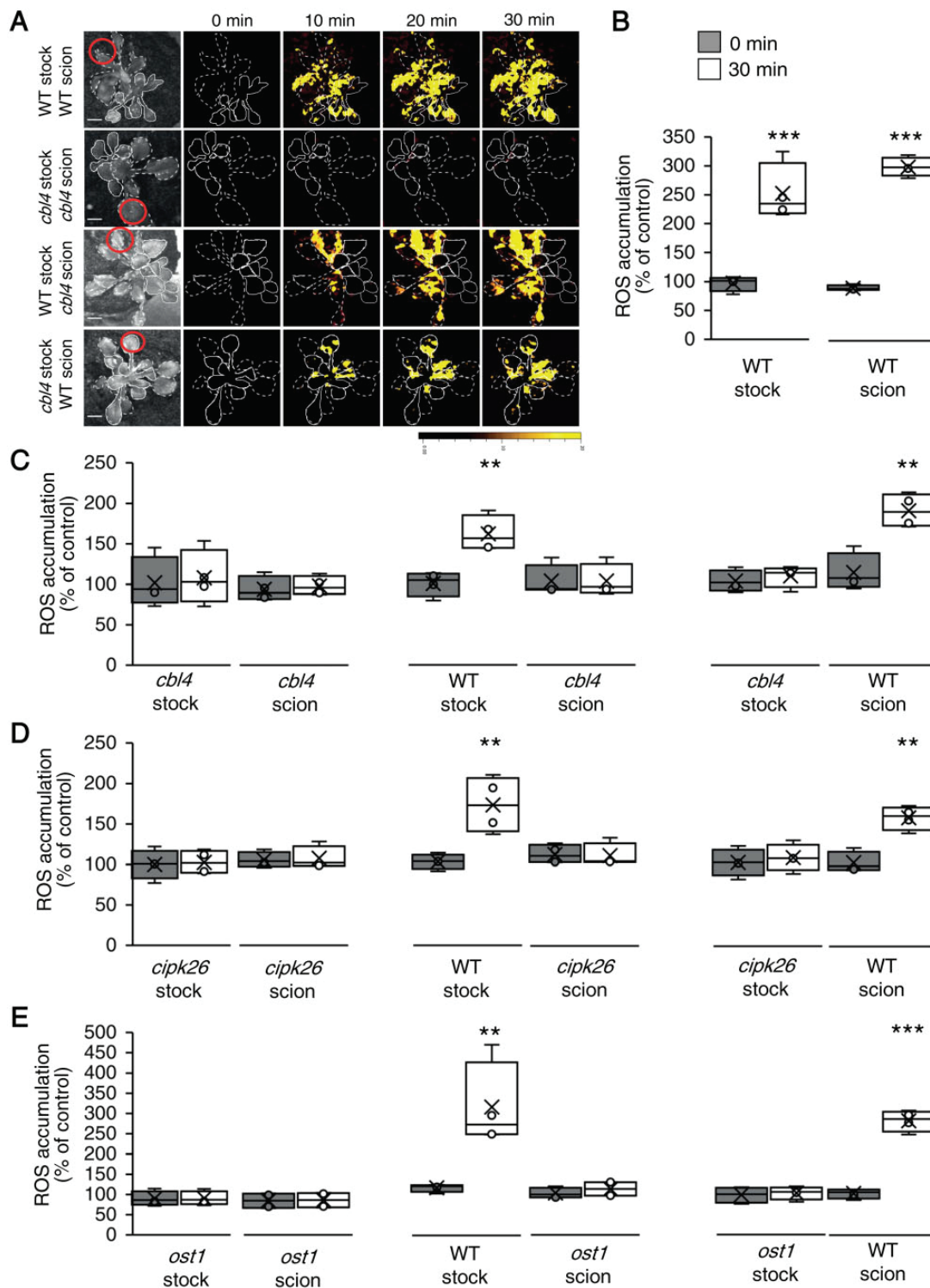
Figure 8 CBL4, CIPK26, and OST1 are required for systemic ROS signal propagation, but not initiation, in response to light stress. A , Representative time-lapse images of ROS accumulation in stock and scion parts of grafted plants, generated using WT and cbl4-1 plants, in response to a local HL stress treatment applied to a single leaf (indicated with a circle) belonging to the stock part. Scions are indicated by solid white lines, and stocks are indicated by dashed white lines. B , Bar graphs showing the combined data from the stock and scion of grafted WT plants subjected to HL stress on a single leaf of the stock scion. C , Same as (B), but for different grafting combinations between WT and cbl4-1 plants. D , Same as (B), but for different grafting combinations between WT and cipk26-2 plants. E , Same as (B), but for different grafting combinations between WT and ost1-2 plants. All experiments were repeated at least three times with 10 plants of each genotype per experiment. ROS accumulation was imaged using H 2 DCFDA. Data are presented as box plot graphs; X is mean \pm SE, N = 30 , ** P < 0.01 , *** P < 0.001 , Student t test. Scale bar, 1 cm.
