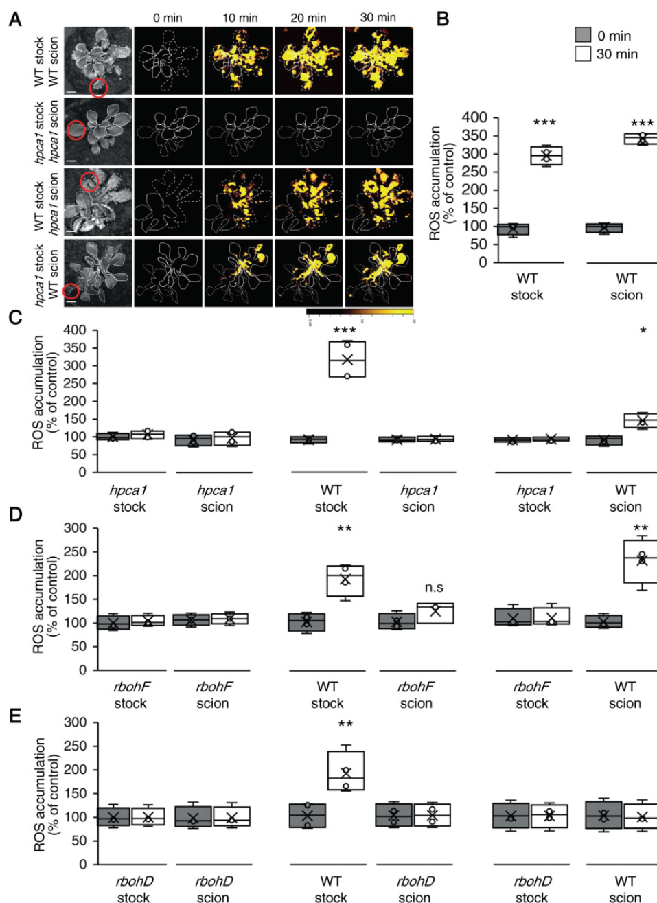
Figure 5 HPCA1 is required for systemic cell-to-cell ROS signal propagation, but not initiation, in response to light stress. A, Representative time-lapse images of ROS accumulation in stock and scion parts of grafted plants, generated using WT and hpca1-1 plants, in response to HL stress applied to a single leaf (indicated with a circle) belonging to the stock part. Scions are indicated by solid white lines, and stocks are indicated by dashed white lines. B, Bar graphs showing the combined data from the stock and scion of grafted WT plants subjected to HL stress on a single leaf of the stock scion. C, Same as (B), but for different grafting combinations between WT and hpca1-1 plants. D, Same as (B), but for different grafting combinations between WT and rbohF plants. E, Same as (B), but for different grafting combinations between WT and rbohD plants. Representative time-lapse images of ROS accumulation in stock and scion parts of grafted WT and rbohD , or rbohF , plants are shown in Supplementary Figure S2 . All experiments were repeated at least three times with 10 plants of each genotype per experiment. ROS accumulation was imaged using H_2DCFDA . Data are presented as box plot graphs; X is mean \pm SE, N = 30 , * P < 0.05 , ** P < 0.01 , *** P < 0.001 , Student's t test. Scale bar, 1 cm.
