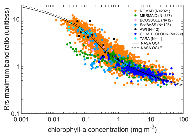
Figure 11. A remote-sensing reflectance maximum band ratio (as defined in text) [[443,490,510]/555] or [[443,490,510]/560] if 555 not available) as a function of chlorophyll- a concentration. All chlorophyll data were considered, but for a given station, HPLC data were selected if available. Data within 2 nm of the wavelengths were used. For reference, the solid and dotted lines show the NASA OC4 and OC4E v6 standard algorithms, respectively ( https://oceancolor.gsfc.nasa.gov/atbd/chlor_a/ , last access: 18 December 2022). The total number of points was 3645, of which 80 % were from NOMAD.
