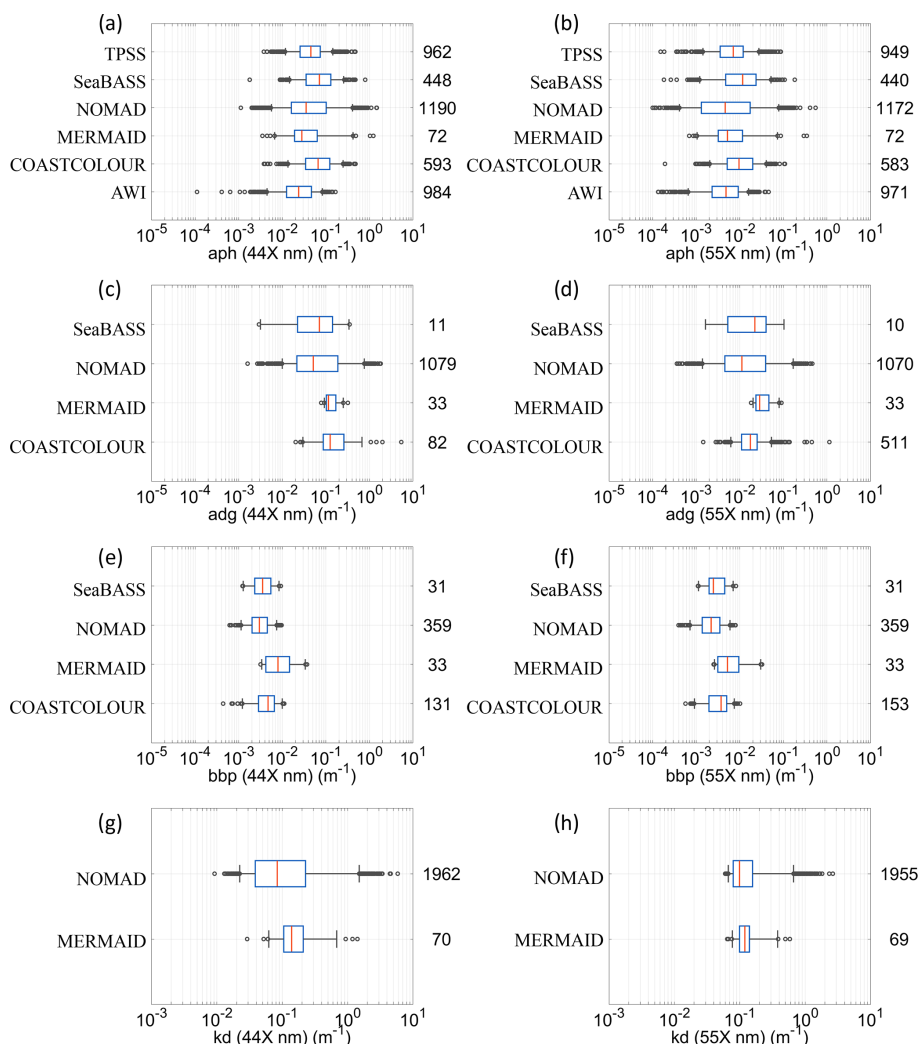
Figure 12. The distribution of: (a) “aph” at 44X nm; (b) “aph” at 55X; (c) “adg” at 44X nm; (d) “adg” at 55X; (e) “bbp” at 44X nm; (f) “bbp” at 55X; (g) “kd” at 44X nm; (h) “kd” at 55X nm. Data were first searched at 445 and 555 nm, and then with a search window up to 8 nm, to include data at 547 nm. The graphical convention is identical to Fig. 2.
