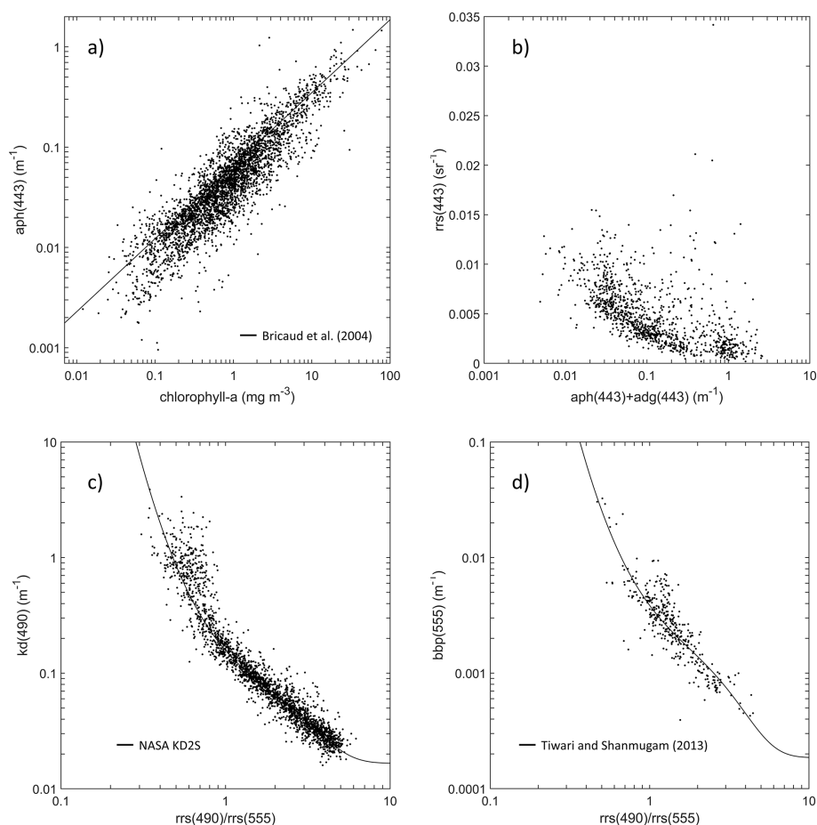
Figure 16. Examples of bio-optical relationships in the final merged table: (a) \text{aph}(443) versus chlorophyll- a . Total number of points (3387) is divided between AWI (753), COASTCOLOUR (335), MERMAID (214), NOMAD (991), SeaBASS (139), and TPSS (955). For reference, the solid line shows the regression from Bricaud et al. (2004). (b) [\text{aph}(443) + \text{adg}(443)] versus \text{rrs}(443) . Total number of points (1112) is divided between MERMAID (33) and NOMAD (1079). (c) [\text{rrs}(490) / \text{rrs}(555)] versus \text{kd}(490) . The total number of points (2280) is divided between MERMAID (62), NOMAD (2117), and SeaBASS (101). For reference, the solid line shows the NASA KD2S standard algorithm ( https://oceancolor.gsfc.nasa.gov/atbd/kd/ , last access: 18 December 2022). (d) [\text{rrs}(490) / \text{rrs}(555)] versus \text{bbp}(555) . The total number of points (365) is divided between MERMAID (33), NOMAD (324), COASTCOLOUR (4), and SeaBASS (4). For reference, the solid line shows the relation proposed by Tiwari and Shanmugam (2013). A search window of 2 nm was used for (a) and (b) , and a search window of 5 nm was used for (c) and (d) to include data at 560 nm when not available at 555 nm.
