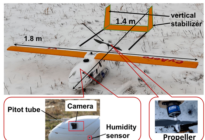
Fig. 1. The fixed-wing UAV used in the present study.
