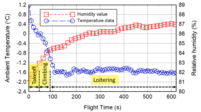
Fig. 4. Time evolution of the ambient temperature and relative humidity (RH) values measured by the onboard sensors during flight mission #2.
