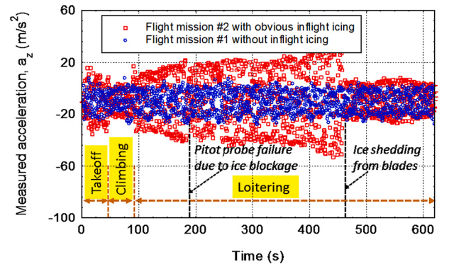
Fig. 12. Comparison of the measured acceleration data during the two flight missions.
