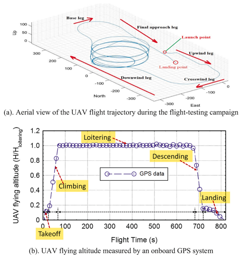
Fig. 3. The measured flight trajectory during the UAV flight-testing campaign.
