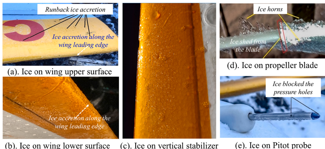
Fig. 6. Snapshot images of the ice structures accreted on the UAV airframe surface acquired right after the UAV landed on the ground.
