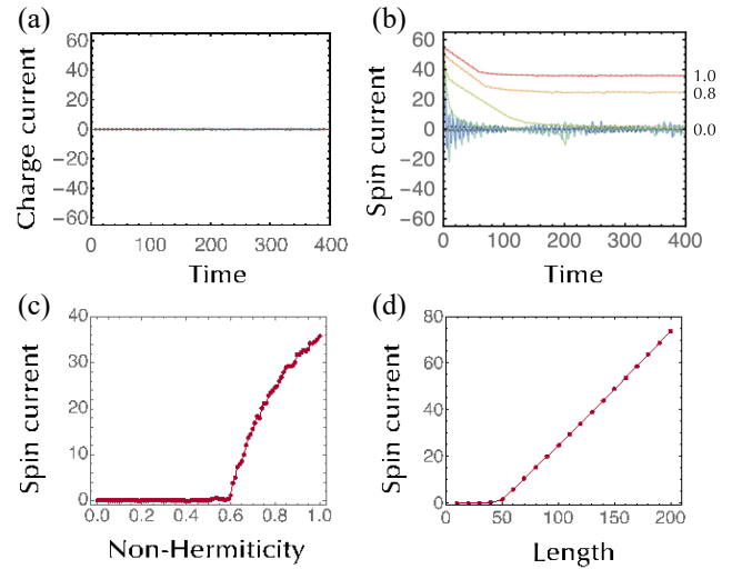
FIG. 10. Current in the symplectic Hatano-Nelson model with open boundaries ( J \approx 1.0 , \Delta \approx 0.5 ). The initial state is prepared as Eq. (24). Time evolution of the (a) charge current I_c \approx \langle \hat{c}_l^\dagger \hat{c}_{l+1} \rangle and (b) spin current I_s \approx \langle \hat{c}_l^\dagger \hat{\sigma}_l \hat{c}_{l+1} \rangle for L \approx 100 and \gamma \approx 0.0, 0.2, 0.4, 0.5, 0.6, 0.8, 1.0 . (c) Spin current for the steady state as a function of non-Hermiticity \gamma for L \approx 100 . (d) Spin current for the steady state as a function of the system length L for \gamma \approx 0.8 .
