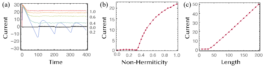
FIG. 4. Total charge current I \hat{\sigma}_t = \sum_{l=1}^{L-1} I_l \hat{\sigma}_t in the Hatano-Nelson model with open boundaries ( J = 1.0 ). The initial state is prepared as the charge density wave state in Eq. (4). (a) Time evolution of the current ( L = 100 ) for \gamma = 0.0 (black dashed curve), 0.2 (blue curve), 0.4 (green curve), 0.6 (light green curve), 0.8 (orange curve), and 1.0 (red curve). (b) Charge current for the steady state as a function of non-Hermiticity \gamma for L = 100 . (c) Charge current for the steady state as a function of the system length for \gamma = 0.8 .
