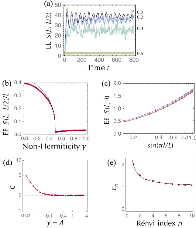
FIG. 14. Entanglement entropy of the symplectic Hatano-Nelson model with periodic boundaries ( L \approx 100 , J \approx 1.0 ). The initial state is prepared as Eq. (24). (a) Time evolution of the entanglement entropy S(L, L/2) ( \Delta \approx 0.5 ) for \gamma \approx 0.0 (black dashed curve), 0.2 (blue curve), 0.4, 0.5, 0.6 (green curves), 0.8 (orange curve), and 1.0 (red curve). (b) Entanglement entropy density S(L, L/2)/L for the steady state as a function of non-Hermiticity \gamma ( \Delta \approx 0.5 ). The black dashed curve is the fitting result S(L, L/2)/L \approx 0.56\delta\Delta/J - \gamma/J^{0.33} around the critical point \gamma \approx \Delta . (c) Entanglement entropy S(L, l) for the steady state at the critical point ( \gamma \approx \Delta ) as a function of the subsystem length l for \gamma \approx 0.0, 0.1, 0.2, 0.4, 0.6, 0.8 , and 1.0. (d) Effective central charge c as a function of \gamma at the critical point ( \gamma \approx \Delta ). The black dashed line shows c \approx 2 . (e) c_n obtained from the Rényi entanglement entropy S_n^{\text{Rényi}}(L, l) for the steady state at the critical point ( \gamma \approx \Delta \approx 1.0 ) as a function of the Rényi index n . The black dashed curve shows the conformal field theory result c_n \approx c\delta 1/p - 1/np=2 with c \approx 2 .
