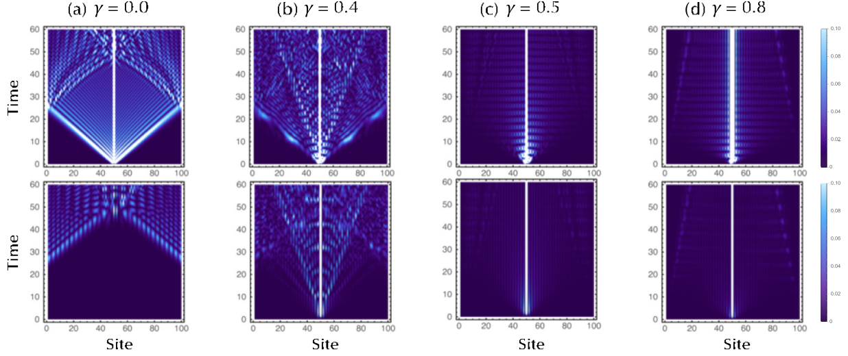
FIG. 9. Correlation propagation in the symplectic Hatano-Nelson model with open boundaries ( L \approx 100 , J \approx 1.0 ; \Delta \approx 0.5 ). The absolute values |C_{l\uparrow,l\uparrow}| (top panels) and |C_{l\uparrow,l\downarrow}| (bottom panels) of the correlation matrix are shown as a function of site l and time t with l_0 \approx L/2 \approx 50 . The initial state is prepared as Eq. (24). Non-Hermiticity is chosen to be (a) \gamma \approx 0.0 , (b) \gamma \approx 0.4 , (c) \gamma \approx 0.5 , and (d) \gamma \approx 0.8 .
