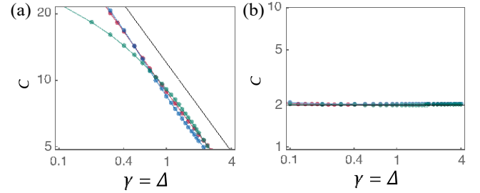
FIG. 16. Effective central charge c of the symplectic Hatano-Nelson model ( L \approx 100 , J \approx 1.0 ) at the critical point ( \gamma \approx \Delta ) under the (a) open boundary conditions and (b) periodic boundary conditions. For each \gamma \approx \Delta , the effective central charge c is obtained from the logarithmic scaling of the steady-state entanglement entropy for the initial states in Eq. (24) (red dots), Eq. (C1) (blue dots), and Eq. (C2) (green dots). The black dashed lines are (a) c \approx \gamma^{-2/3} and (b) c \approx 2 .
