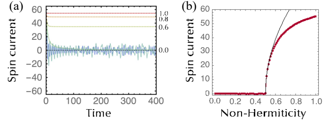
FIG. 13. Spin current in the symplectic Hatano-Nelson model with periodic boundaries ( L \sim 100 , J \sim 1.0 , \Delta \sim 0.5 ). The initial state is prepared as Eq. (24). (a) Time evolution of the spin current for \gamma \sim 0.0 (black dashed curve), 0.2 (blue curve), 0.4, 0.5, 0.6 (green curves), 0.8 (orange curve), and 1.0 (red curve). (b) Spin current for the steady state as a function of non-Hermiticity \gamma . The black dashed curve is the fitting result I_s \sim 123J\delta\gamma = J - \Delta = J\delta\gamma^{0.50} around the critical point \gamma \sim \Delta .
