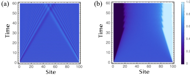
FIG. 2. Time evolution of the local particle number n_l(t) in the Hatano-Nelson model with open boundaries ( L = 100 , J = 1.0 ) for (a) \gamma = 0.0 and (b) \gamma = 0.8 . The initial state is prepared as the charge density wave state in Eq. (4). In the presence of non-Hermiticity, particles accumulate at the boundary, which is a clear signature of the non-Hermitian skin effect.
