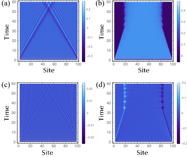
FIG. 5. Local current distribution in the Hatano-Nelson model with open boundaries ( J \approx 1.0 ). The initial state is prepared as the charge density wave state in Eq. (4). (a),(b) Time evolution of the local current I_{\delta t P} \approx h\psi_{\delta t P} j_l \psi_{\delta t P}^* for (a) \gamma \approx 0.0 and (b) \gamma \approx 0.8 . (c),(d) Time evolution of the local particle inflow for (c) \gamma \approx 0.0 and (d) \gamma \approx 0.8 .
