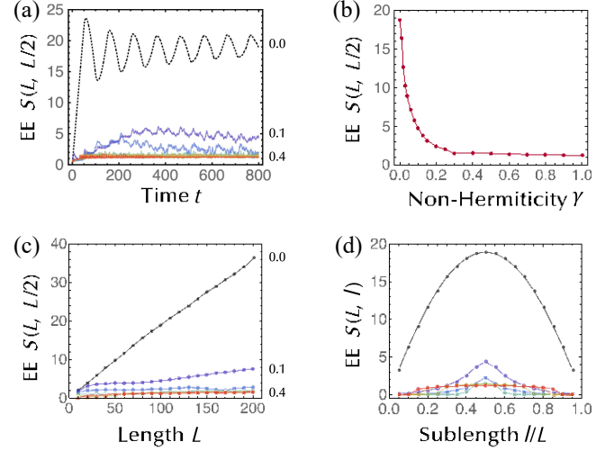
FIG. 6. Entanglement entropy (EE) of the Hatano-Nelson model with open boundaries ( J \approx 1.0 ). The initial state is prepared as the charge density wave state in Eq. (4). (a) Time evolution of the entanglement entropy S_{\delta L; L=2P} ( L \approx 100 ) for \gamma \approx 0.0 (black dashed curve), 0.1 (violet curve), 0.2 (blue curve), 0.4 (green curve), 0.6 (light green curve), 0.8 (orange curve), and 1.0 (red curve). (b) Entanglement entropy S_{\delta L; L=2P} for the steady state as a function of non-Hermiticity \gamma ( L \approx 100 ). (c) Entanglement entropy S_{\delta L; L=2P} for the steady state as a function of the system length L . (d) Entanglement entropy S_{\delta L; \mathbb{P}} ( L \approx 100 ) for the steady state as a function of the subsystem length l .
