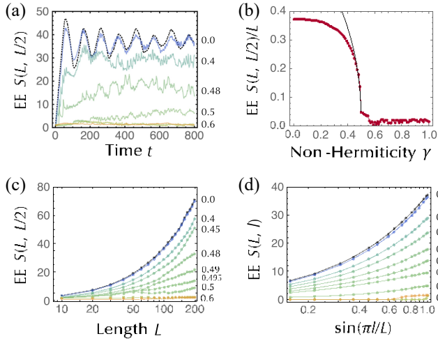
FIG. 11. Entanglement entropy of the symplectic Hatano-Nelson model with open boundaries ( J \approx 1.0 , \Delta \approx 0.5 ). The initial state is prepared as Eq. (24). (a) Time evolution of the entanglement entropy S(L, t) ( L \approx 100 ) for \gamma \approx 0.0 (black dashed curve), 0.2 (blue curve), 0.4, 0.48, 0.5 (green curves), 0.6 (light green curve), and 0.8 (orange curve). (b) Entanglement entropy density S(L, L) ( L \approx 100 ) for the steady state as a function of non-Hermiticity \gamma . The black dashed curve is the fitting result S(L, L) \approx 0.94 \ln \Delta - \gamma \ln \Delta^{0.44} around the critical point \gamma \approx \Delta . (c) Entanglement entropy S(L, L) for the steady state as a function of the system length L for \gamma \approx 0.0, 0.2, 0.4, 0.45, 0.48, 0.49, 0.495, 0.5, 0.6 , and 0.8. (d) Entanglement entropy S(L, l) ( L \approx 100 ) for the steady state as a function of the subsystem length l .
