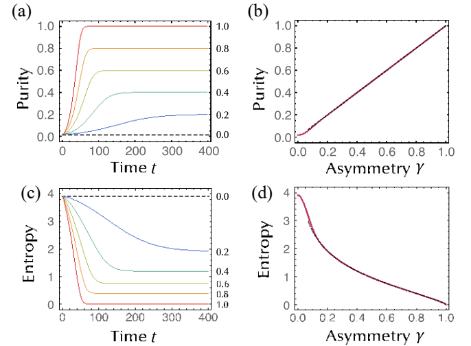
FIG. 15. Purification induced by the Liouvillian skin effect ( L = 50, J = 1.0 ). The initial state is prepared as the completely mixed state \rho_0 \equiv 1/L with the purity P_0 \equiv 1/L and the von Neumann entropy S_0 \equiv \log L . (a) Time evolution of the purity for \gamma = 0.0 (black dashed curve), \gamma = 0.2 (blue curve), \gamma = 0.4 (green curve), \gamma = 0.6 (light green curve), \gamma = 0.8 (orange curve), and \gamma = 1.0 (red curve). (b) Steady-state purity as a function of \gamma (red curve), consistent with the analytical result P_s \equiv \gamma/J (black dashed curve). (c) Time evolution of the von Neumann entropy. (d) Steady-state von Neumann entropy as a function of \gamma (red curve), consistent with the analytical result S_s \equiv \log J - \gamma \log J - \gamma \log \gamma - \gamma \log (J - \gamma) (black dashed curve).
