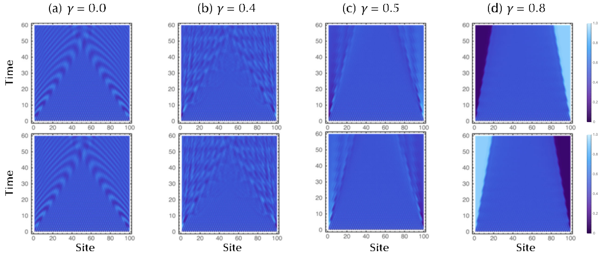
FIG. 8. Time evolution of the local particle number n_{i;s}(\vec{t}) = \langle \psi | \hat{n}_{i;s}(\vec{t}) | \psi \rangle for s = \uparrow (top panels) and s = \downarrow (bottom panels) in the symplectic Hatano-Nelson model with open boundaries ( L = 100 , J = 1.0 , \Delta = 0.5 ). The initial state is prepared as Eq. (24). Non-Hermiticity is chosen to be (a) \gamma = 0.0 , (b) \gamma = 0.4 , (c) \gamma = 0.5 , and (d) \gamma = 0.8 . While no skin effect occurs for |\gamma| < j\Delta j , the reciprocal skin effect occurs for |\gamma| > j\Delta j .
