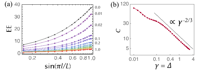
FIG. 12. Entanglement entropy of the symplectic Hatano-Nelson model with open boundaries ( J \approx 1.0 ) at the critical point ( \gamma \approx \Delta ). The initial state is prepared as Eq. (24). (a) Entanglement entropy S(L, l) ( L \approx 100 ) for the steady state as a function of the subsystem length l for \gamma \approx 0.0, 0.01, 0.02, 0.05, 0.1, 0.2, 0.3, 0.4, 0.5, 0.6, 0.7, 0.8, 0.9 , and 1.0. (b) Effective central charge c as a function of \gamma \approx \Delta ( L \approx 100 ).
