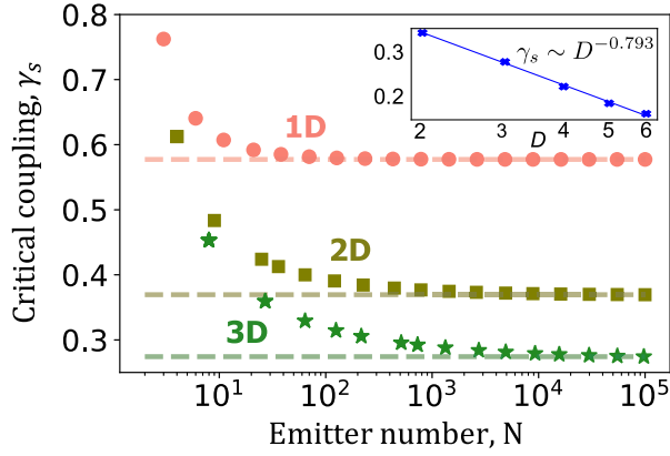
FIG. 4. Critical coupling \gamma_s for exponentially decaying interactions in a 1D chain, a 2D square array, and a 3D cubic array with N emitters. Superradiance occurs for \gamma > \gamma_s . For all dimension D , \gamma_s becomes independent of N for large N . Inset: log-log plot of \gamma_s against D for N \approx 10^6 . \gamma_s decreases as D increases with a power-law scaling \gamma_s \sim D^{-0.793} .
