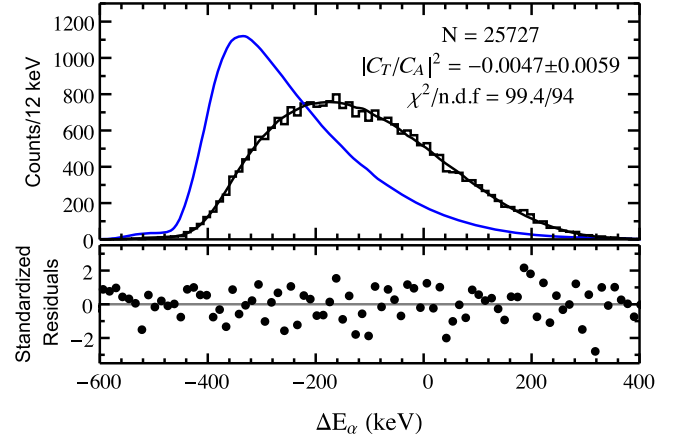
FIG. 2. Energy difference spectrum along with the fit, shown in black, to the simulated spectrum and normalized residuals. Shown in blue is the expected result for a pure tensor interaction. The number of events N , the fitted |C_T/C_A|^2 , and the fit \chi^2 per number of degrees of freedom are also shown.
