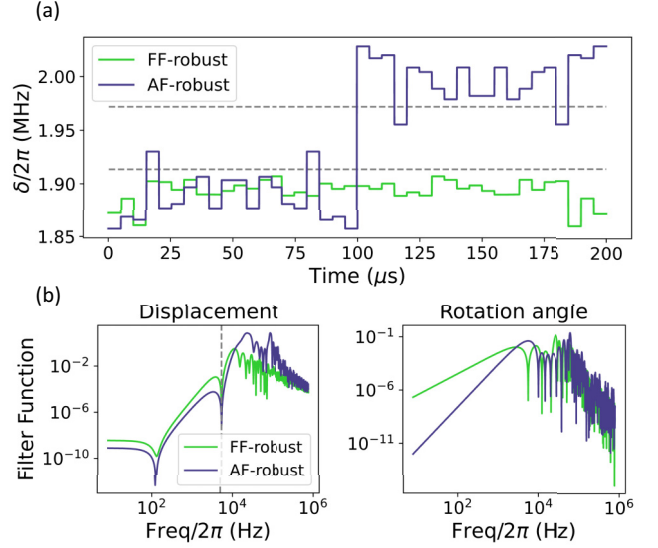
FIG. 7. (a) An example of 200-μs pulses for two-ion discrete FF-robust and AF-robust FM XX(\pi/4) pulses. The carrier Rabi frequencies for the FF- and AF-robust pulses are 73.65 and 100.36 kHz, respectively. (b) The FFs of the pulses in panel (a). The pulses are optimized such that the displacement FF is suppressed near 5 kHz (dashed line).
