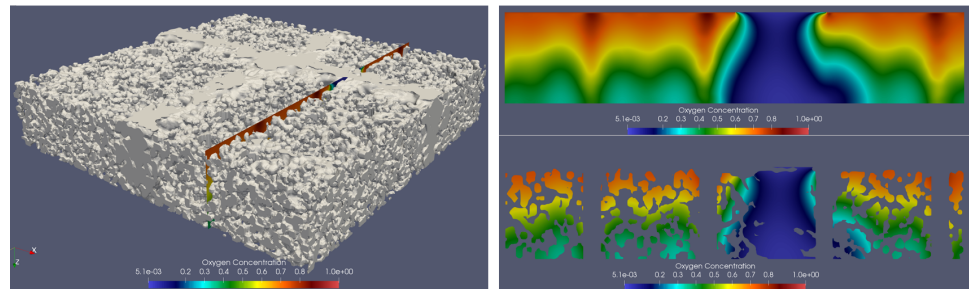
Figure 17. Detailed information about oxygen concentration within the hydrogel for the case with two outlets. (Left): 3D hydrogel with a 2D slice. (Right): A section of the 2D slice through hydrogel containing details of oxygen concentration (top) and hydrogel structure (bottom). Red is high oxygen concentration and dark blue is low oxygen concentration. Maximum oxygen concentration was 1.06 \times 10^{-7} \text{ mol/cm}^3 . The flow is from top to bottom. The dark red colors with high concentration indicate where the ultrafiltrate channels are located.
