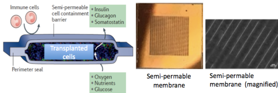
Figure 1. (Left): An illustration of an islet encapsulation device [6]; (Middle): Semi-permeable silicon membrane; (Right): A scanning electron microscope (SEM) image of the membrane surface illustrating slits 2 \mu\text{m} in length and 7 nm is width (courtesy of Dr. Roy).
