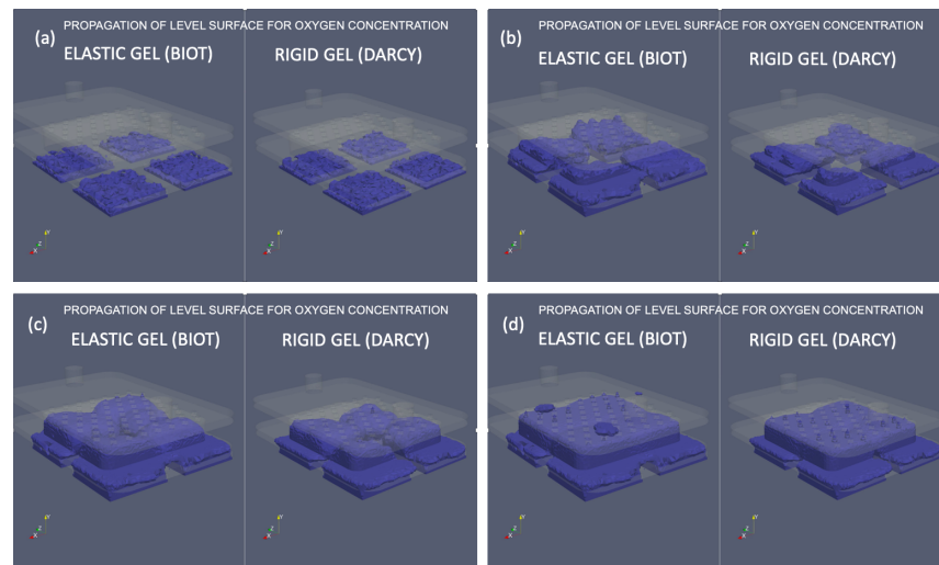
Figure 18. Oxygen front propagation: Comparison between the Biot model (assuming poroelastic hydrogel), and Darcy model (assuming rigid porous hydrogel). The figure shows four snap-shots at increasing times from (a–d) showing the propagation of a level surface of oxygen concentration. In figure (d) we see that oxygen front has already reached the top gasket in the case of the poroelastic Biot model (figure (d) left), while in the case of the rigid gel modeled by Darcy law, the front is still within the islet chamber, not yet reaching the top gasket (figure (d) right).
