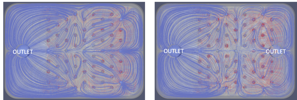
Figure 13. Comparison of the streamlines viewed from the top for the designs with one outlet (left), c.f. Figure 9, and with two outlets (right), c.f. Figure 12. The top view shows the outlets, the slow flow (blue) in the top gasket, and the faster flow (red) in the islet chamber. The same velocity scale was used for both pictures. We see stronger flow through the islet chamber on the right (two outlets). In particular, the transverse flow, away from the ultrafiltrate channels, is much stronger in the case of two outlets. This can also be seen in Figure 12 (bottom). A combination of the presence of the second outlet and the “misalignment between the islet chamber and the two inlet membranes in the right half of the chamber is responsible for the increase in transverse (diagonal) flow.
