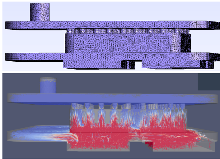
Figure 9. Computational domain and streamlines corresponding to the red box in Figure 4. The inlet is at the bottom through four membranes, and the outlet is at the top through the vertical cylinder. The maximal velocity is 3.5 cm/s (shown in red).
