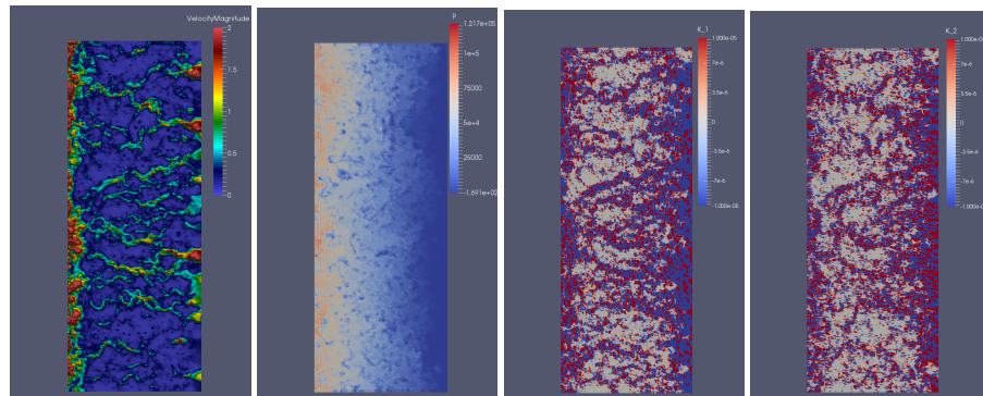
Figure 8. A SPH simulation of a 2D slice of a synthetically generated hydrogel showing: (a) Filtration velocity magnitude ; (b) Pressure field; (c) Hydraulic conductivity coefficient in horizontal direction [\kappa_0]_{11} , and (d) in vertical direction [\kappa_0]_{33} .
