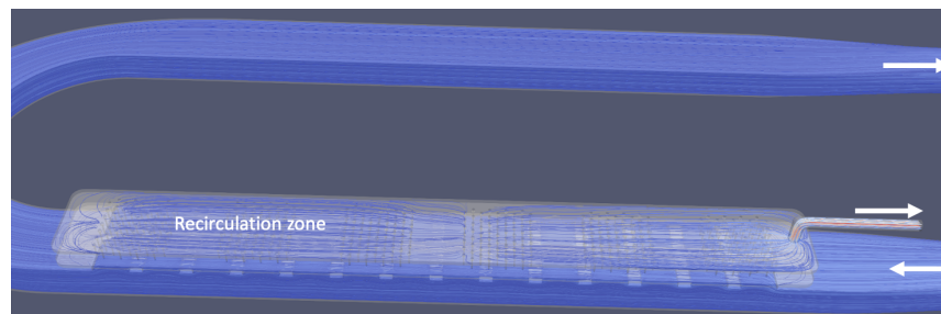
Figure 14. Large recirculation zone in device design with only one outlet.
