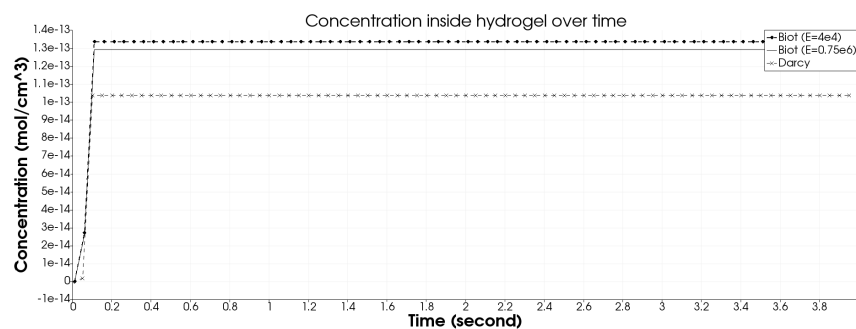
Figure 20. The curves show oxygen concentration over time for three different hydrogels with three different elasticity moduli: alginate hydrogel with Youngs modulus E = 4 \times 10^4 Pascals, alginate with E = 0.75 \times 10^6 Pa, and a very stiff scaffold made of Polycaprolactone (PCL) with E = 1.3 \times 10^8 Pa. We see a significant increase in oxygen concentration for the most elastic alginate hydrogels with E = 4 \times 10^4 Pa and E = 0.75 \times 10^6 Pa over the stiff PLC with E = 1.3 \times 10^8 Pa.
