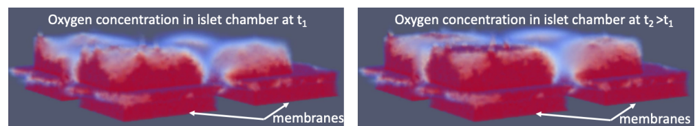
Figure 10. Oxygen concentration at the membranes (inlet) and within the islet chamber for two different times t_1 and t_2 > t_1 as the initial oxygen front convected with the flow enters the bioartificial pancreas. Red denotes high concentration and white and blue low concentration. The flow is from bottom to top. We can see that the regions on the left in both pictures, which are closest to the outlet, get more oxygen than the regions on the right.
