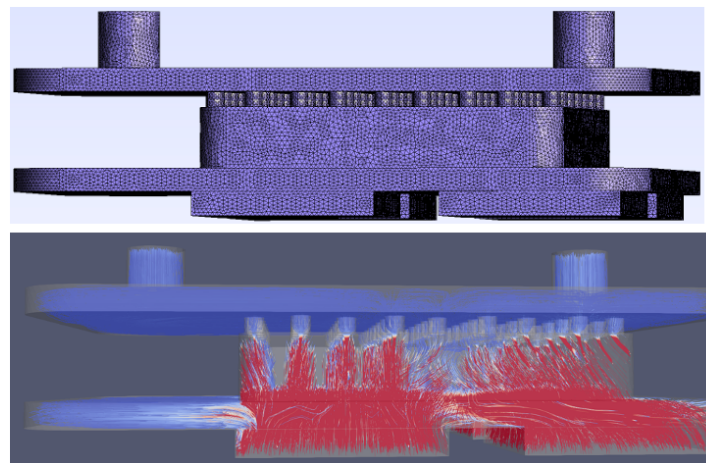
Figure 12. Computational domain and velocity streamlines for the case with two outlets. The maximum velocity is between 3.4 cm/s.
