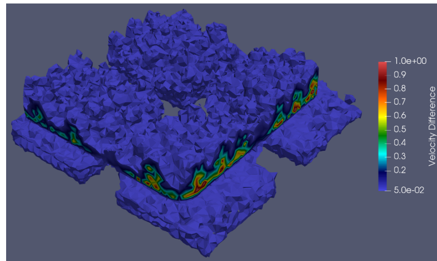
Figure 19. Difference in velocity magnitude between filtration flow through an poroelastic hydrogel, modeled by the Biot model, and rigid hydrogel, modeled by Darcy law. Red is high and blue is low velocity difference. Biot filtration velocity has a higher magnitude, indicating that hydrogel elasticity is conducive to increased filtration flow.
