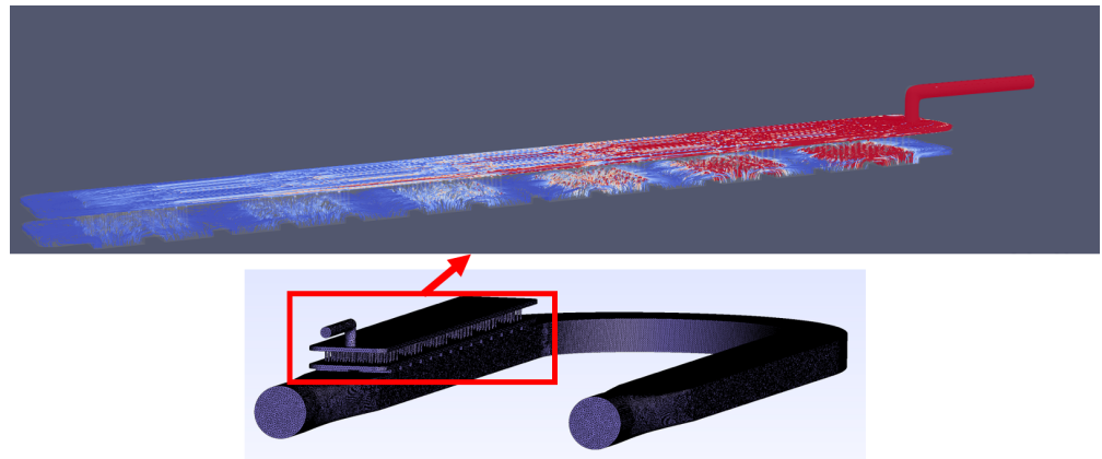
Figure 11. Entire loop. (Top): The colors denote the magnitude of fluid velocity with red denoting high velocity (maximum velocity is equal to 3.5 cm/s) and blue denoting low velocity (minimum velocity is 0 cm/s). (Bottom): The entire computational domain with mesh.
