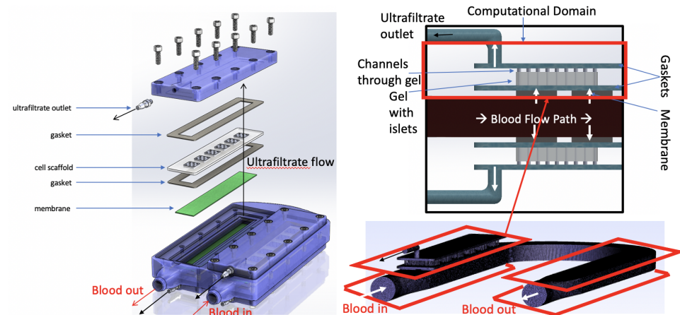
Figure 4. A prototype of a implantable Bioartificial Pancreas Device. The red boxes on the bottom right figure show the location where the four islet chambers are located. Only one of the four chambers is fully depicted in Figure 4 bottom right. A more detailed, magnified sketch of two such chambers is shown on the top figure on the right. The top chamber in the red rectangle shows the computational domain.
