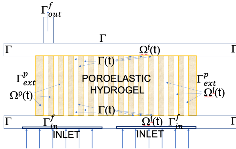
Figure 7. A sketch of a 2D slice of the fluid and poroelastic structure domains together with their boundaries.
