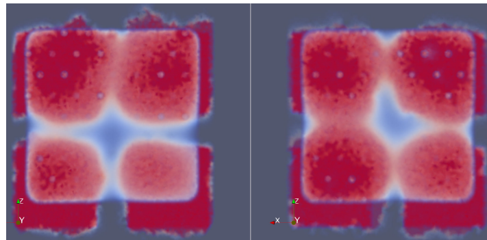
Figure 15. Comparison of oxygen concentration viewed from the top for the designs with one outlet (left), c.f. Figure 9, and with two outlets (right), c.f. Figure 12. The same concentration scale was used for both pictures. High oxygen concentration is shown in red, and low in white and blue. We see larger regions of high oxygen concentration in the figure on the right, corresponding to the design with two outlets. The purple dots are the outlines of the ultrafiltrate channels.
