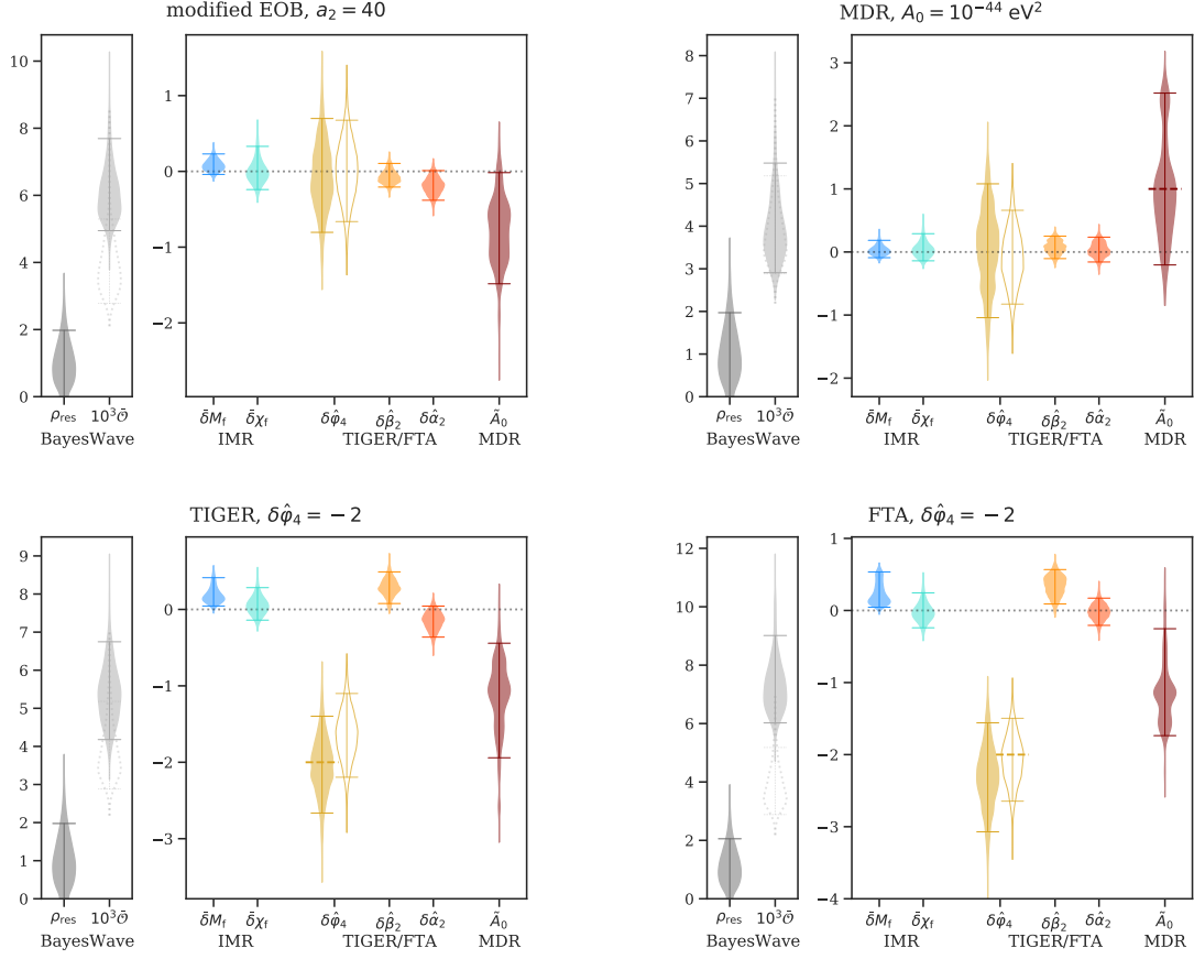
FIG. 5. Like Fig. 4, except for the GW150914-like simulated observations with the smaller GR deviation. Additionally, we are able to scale \tilde{\mathcal{O}} the same way for all cases and also show the corresponding GR distribution in all cases.
